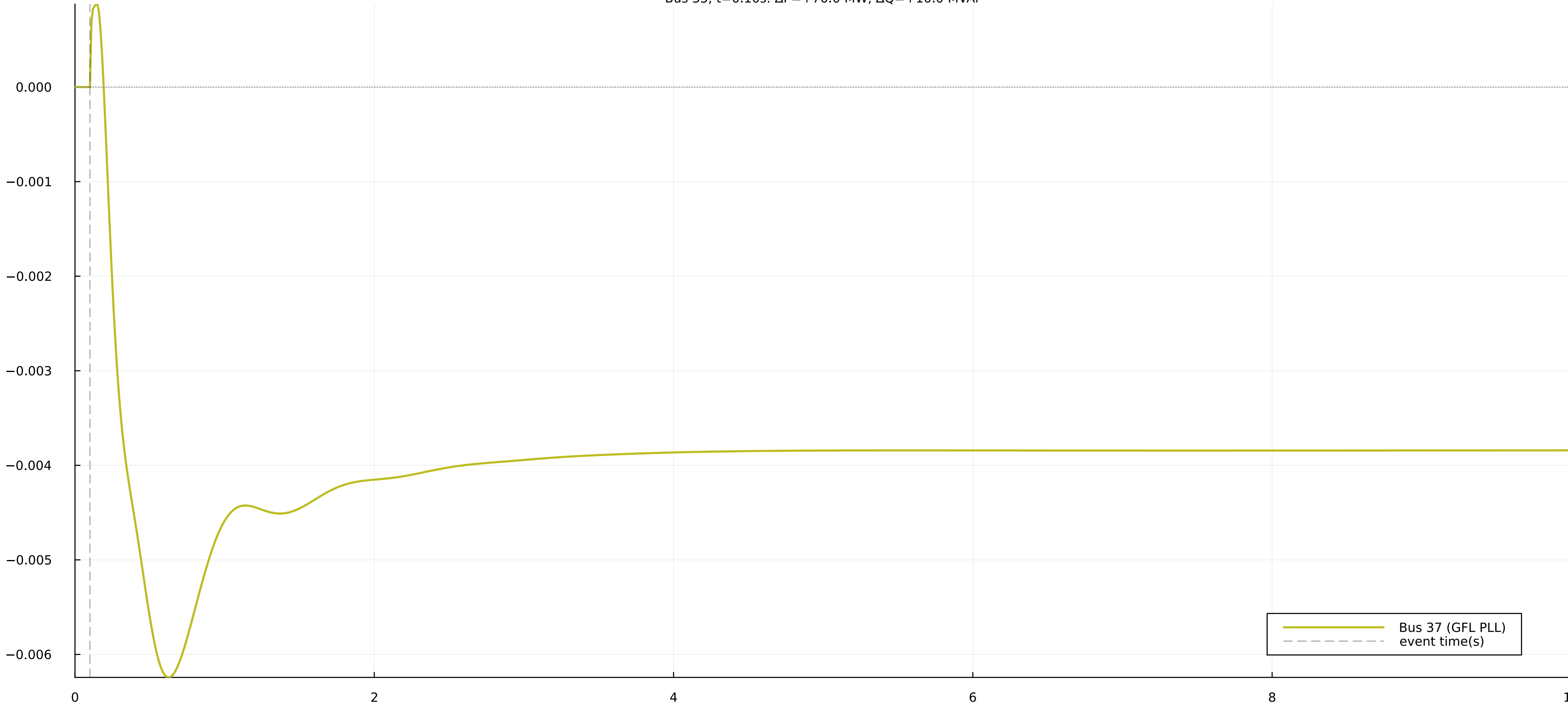
Frequency deviation at bus 37 Bus 35, t=0.10s: \Delta P=+70.0 MW, \Delta Q=+10.0 MVar
