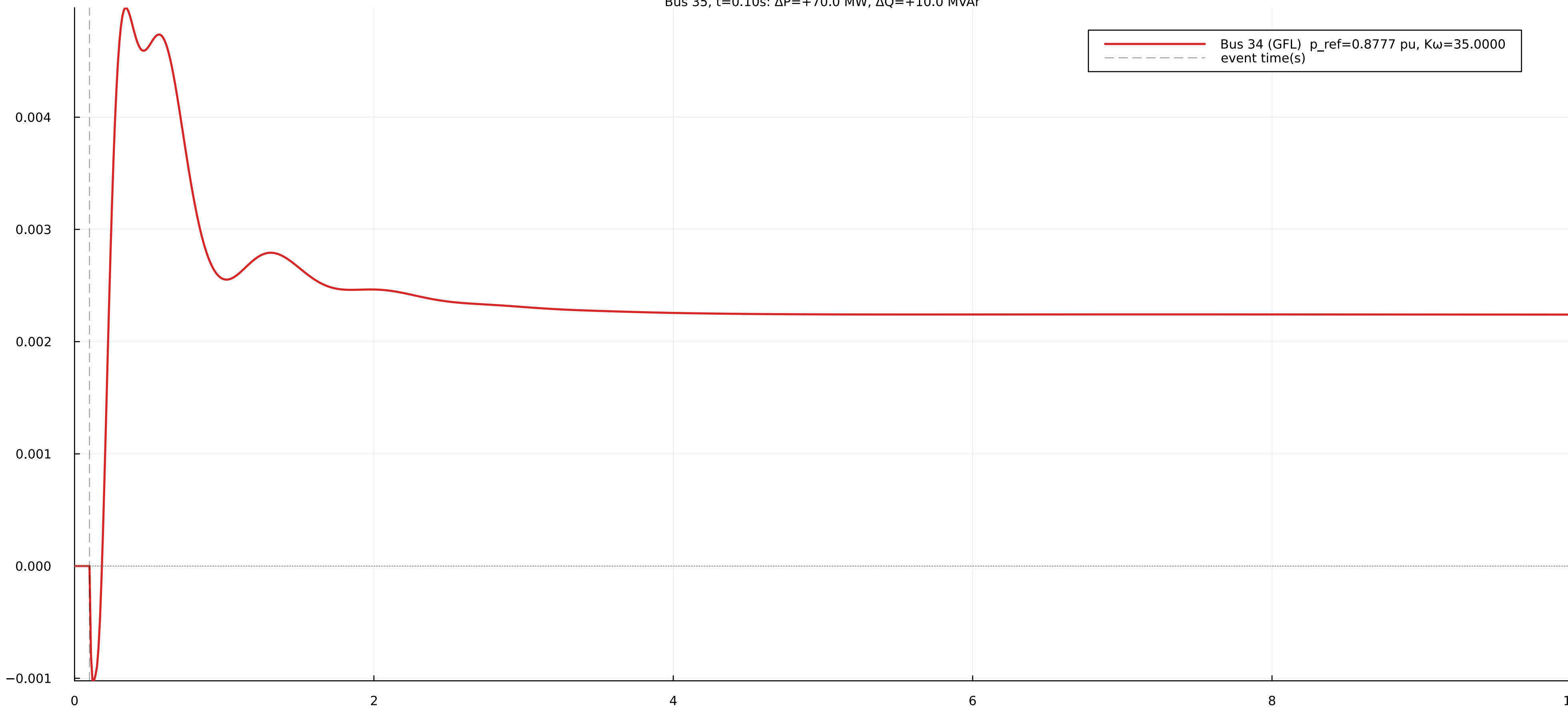
GFL effective P-ref deviation at bus 34 Bus 35, t=0.10s: \Delta P=+70.0 MW, \Delta Q=+10.0 MVar
