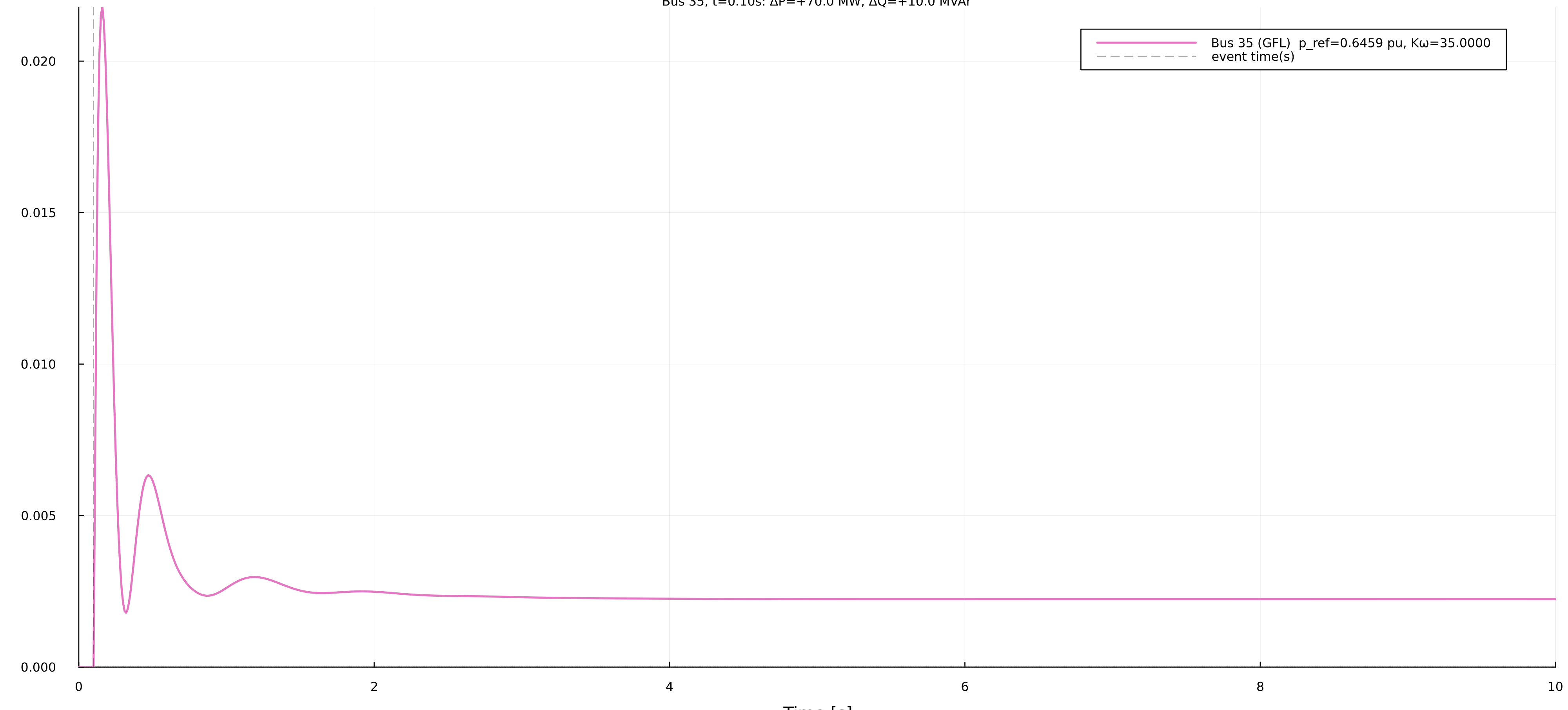
GFL effective P-ref deviation at bus 35 Bus 35, t=0.10s: \Delta P=+70.0 MW, \Delta Q=+10.0 MVar
