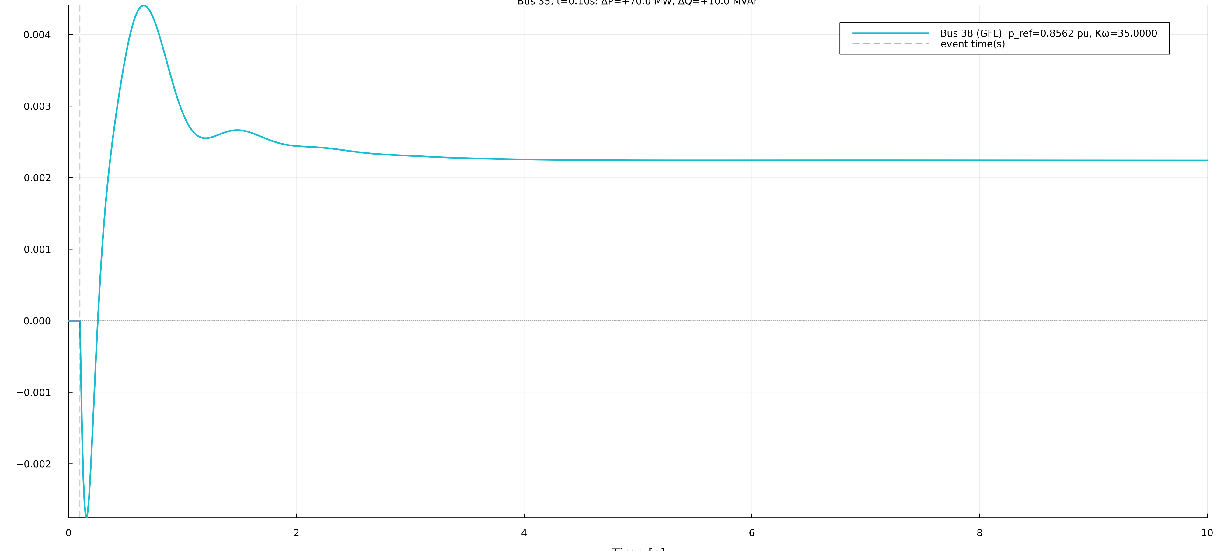
GFL effective P-ref deviation at bus 38 Bus 35, t=0.10s: \Delta P=+70.0 MW, \Delta Q=+10.0 MVar
