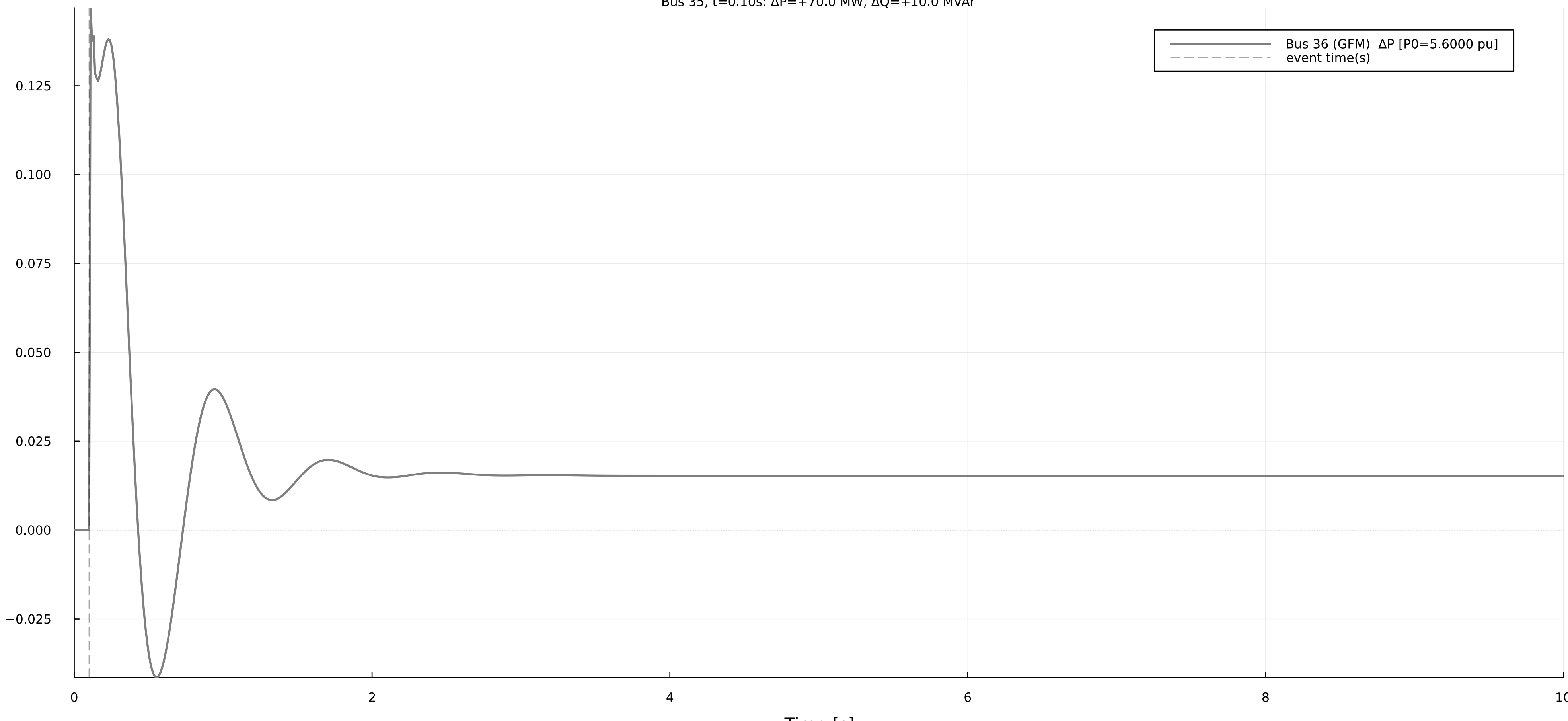
GFM active-power deviation at bus 36 Bus 35, t=0.10s: \Delta P=+70.0 MW, \Delta Q=+10.0 MVar
