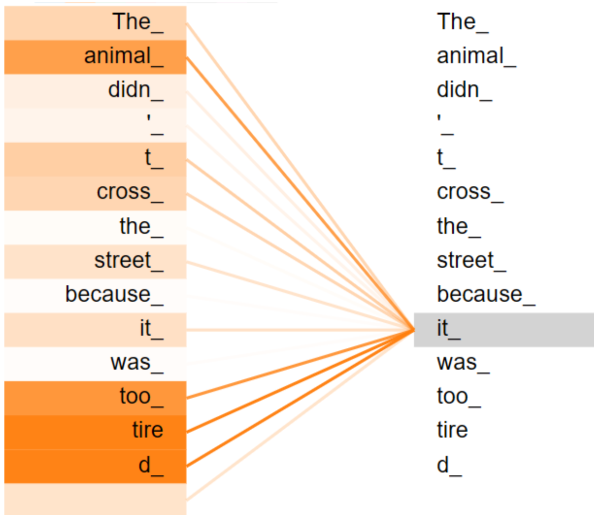
Figure 2.3: Attention Weights of the word “it” in a sentence. Image source
