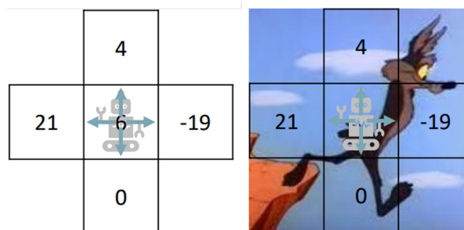
Figure 2.8: State-Value Function
