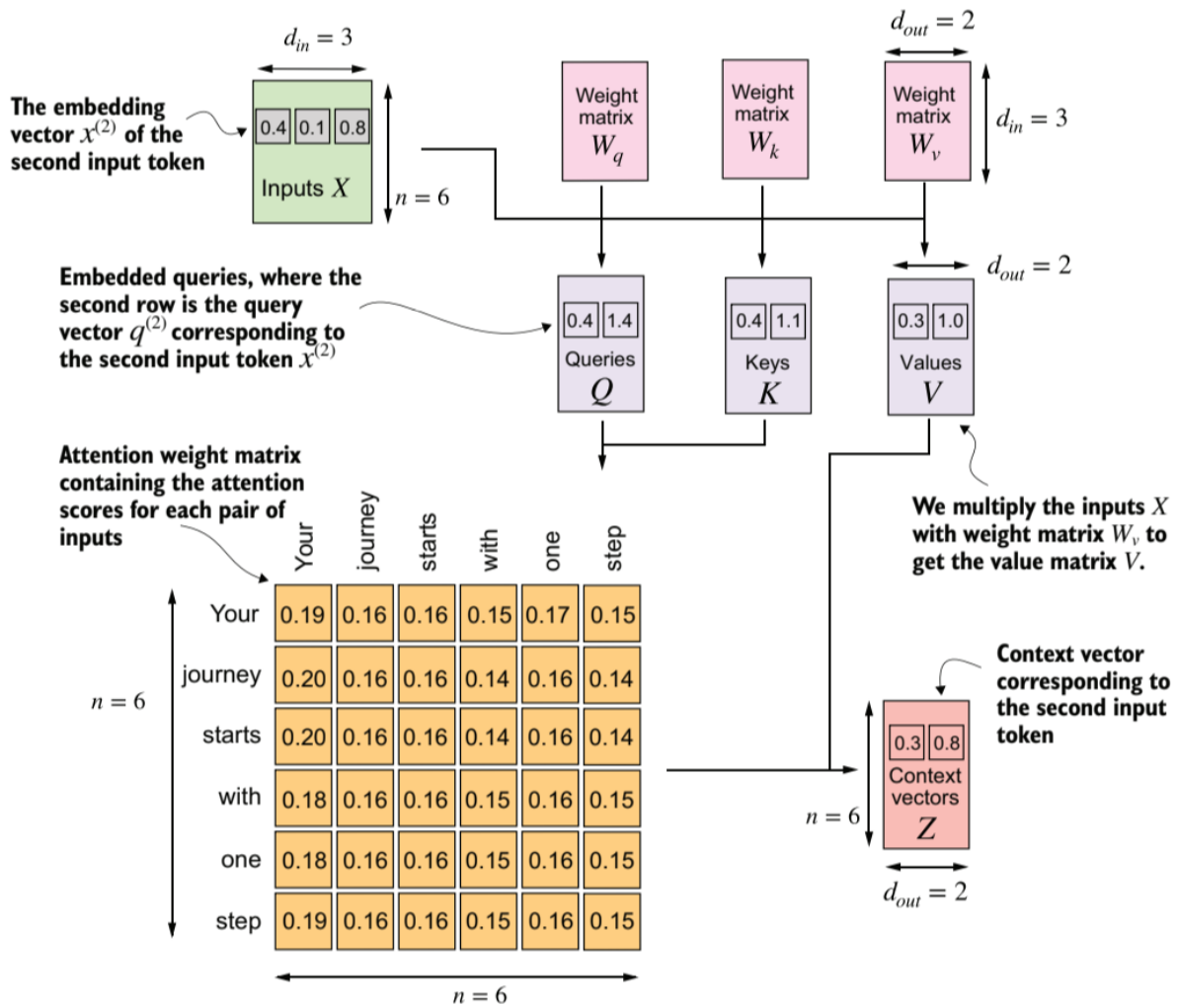
Figure 2.5: Single self-attention Block. Image source [xxx].
