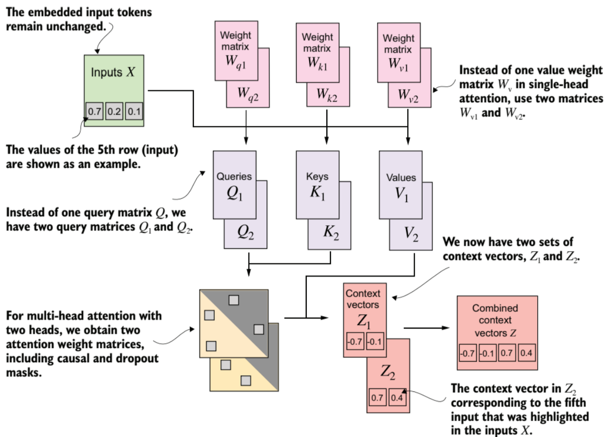
Figure 2.6: Multi-Head Attention Block. Image source [xxx].
