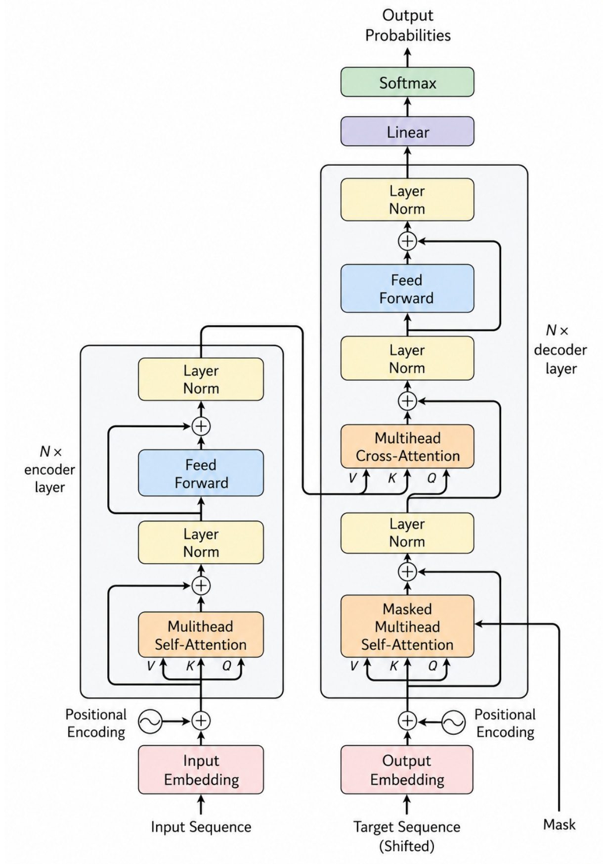
Figure 2.2: Transformer Architecture. Image based on [2].
