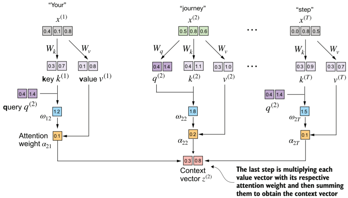
Figure 2.4: Self-attention: Compute the new context vector of each input embedding vector by combining the (attention)-weighted value vectors. Image source [xxx].
