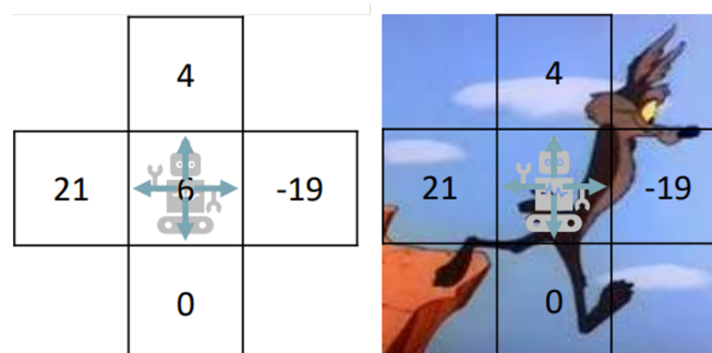
Figure 2.10: State-Value Function
