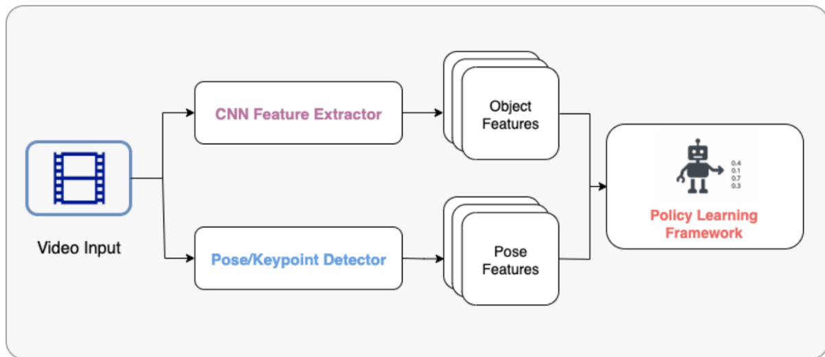
Figure 6.1: Feature Extraction Methods [32].
