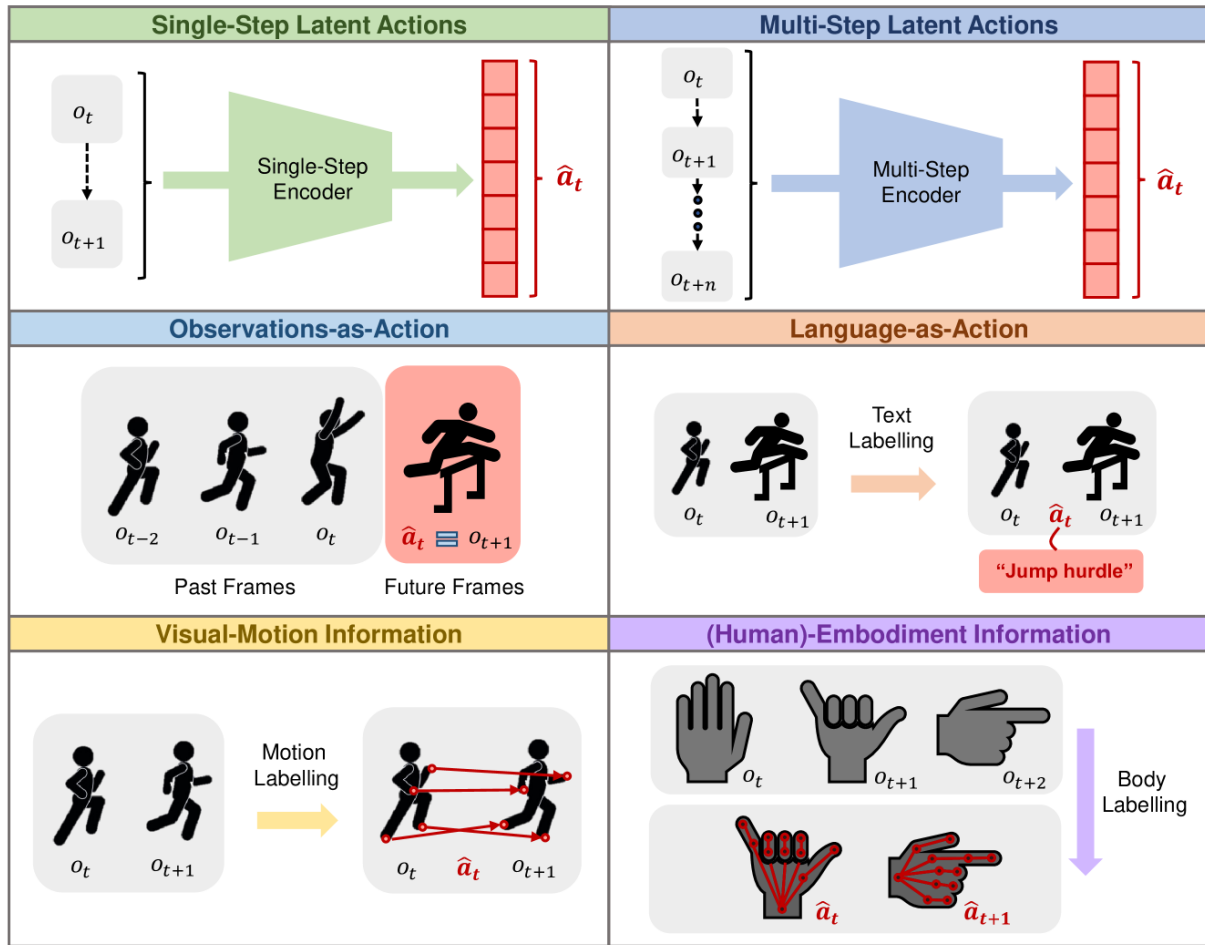
Figure 5.3: Categories of Alternative Action Representations that can be learned or obtained from video data [70].
