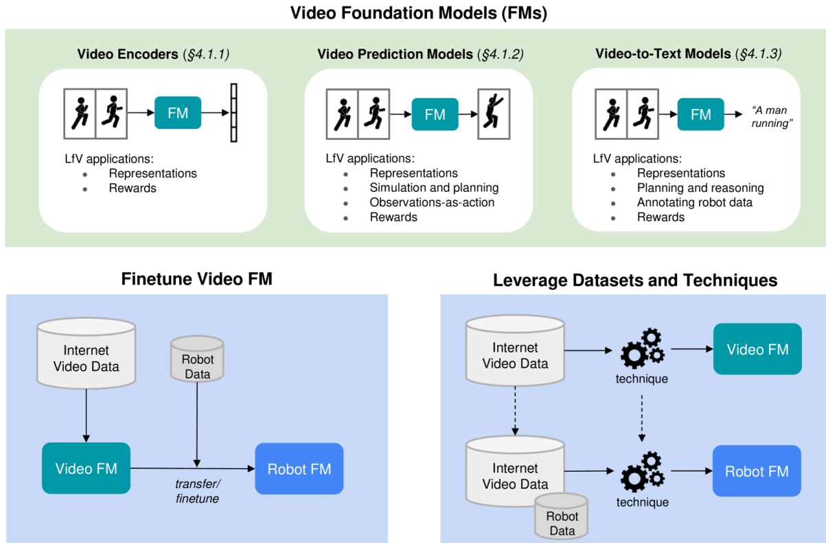
Figure 5.1: Video foundation modelling for Learning from Videos [70].
