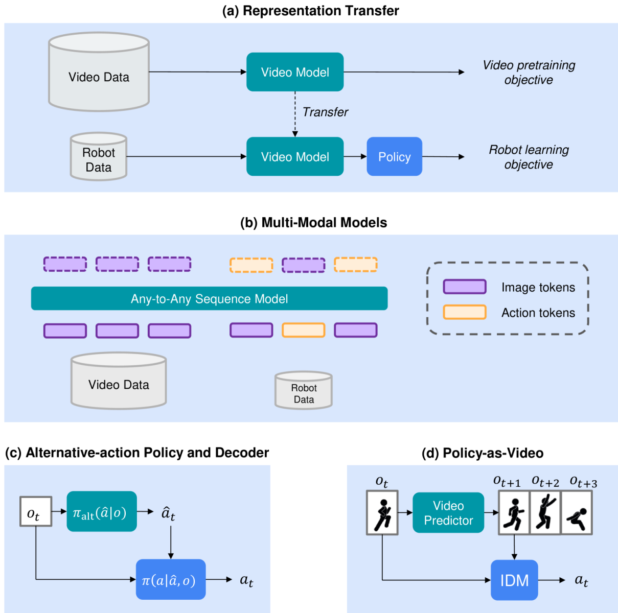
Figure 6.2: Learning Policies from Video [70].
