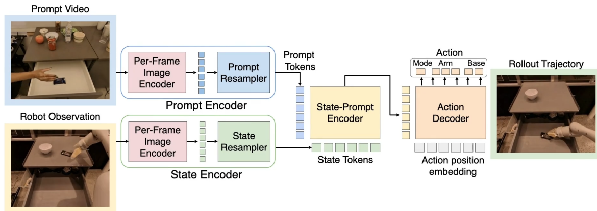
Figure 8.2: Vid2Robot Architecture [?].
