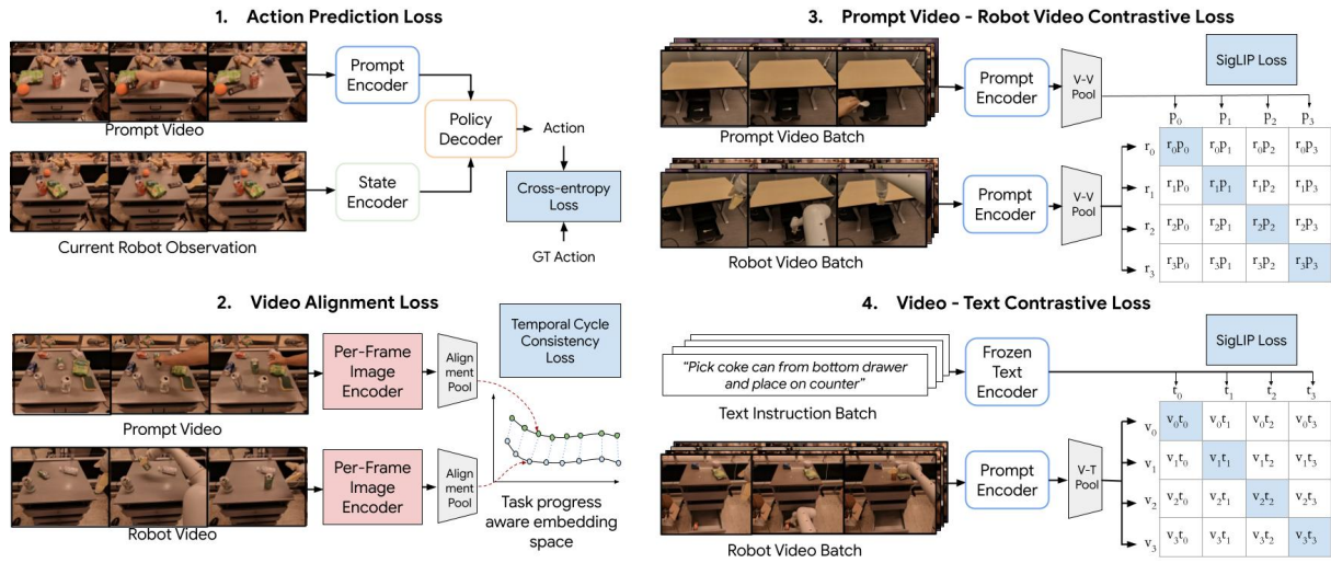
Figure 8.3: Vid2Robot Loss [?].
