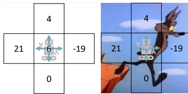
Figure 2.9: State-Value Function
