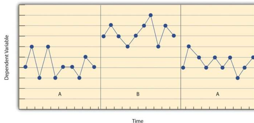
Figure 10.3.1: Results of a Generic Single-Subject Study Illustrating Several Principles of Single-Subject Research
