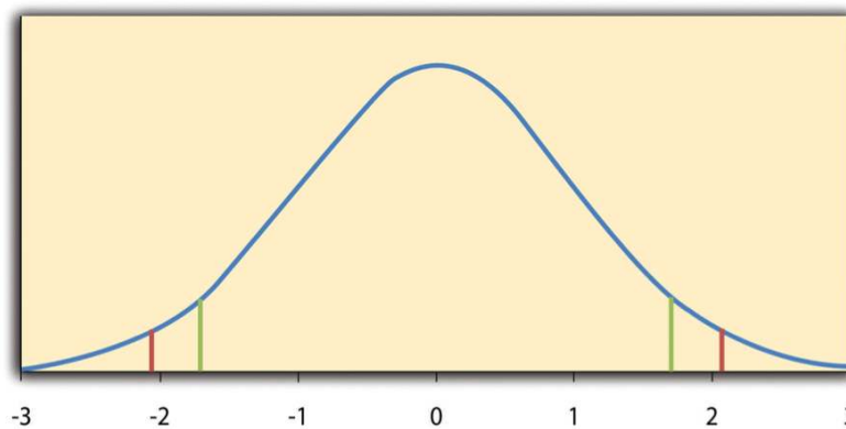
Figure 13.3.1: Distribution of t Scores (With 24 Degrees of Freedom) When the Null Hypothesis Is True. The red vertical lines represent the two-tailed critical values, and the green vertical lines the one-tailed critical values when \alpha = .05 .
