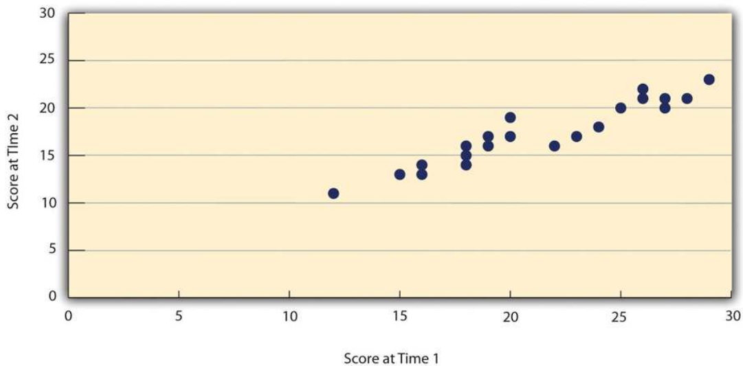
Figure 4.3.1: Test-Retest Correlation Between Two Sets of Scores of Several College Students on the Rosenberg Self-Esteem Scale, Given Two Times a Week Apart
