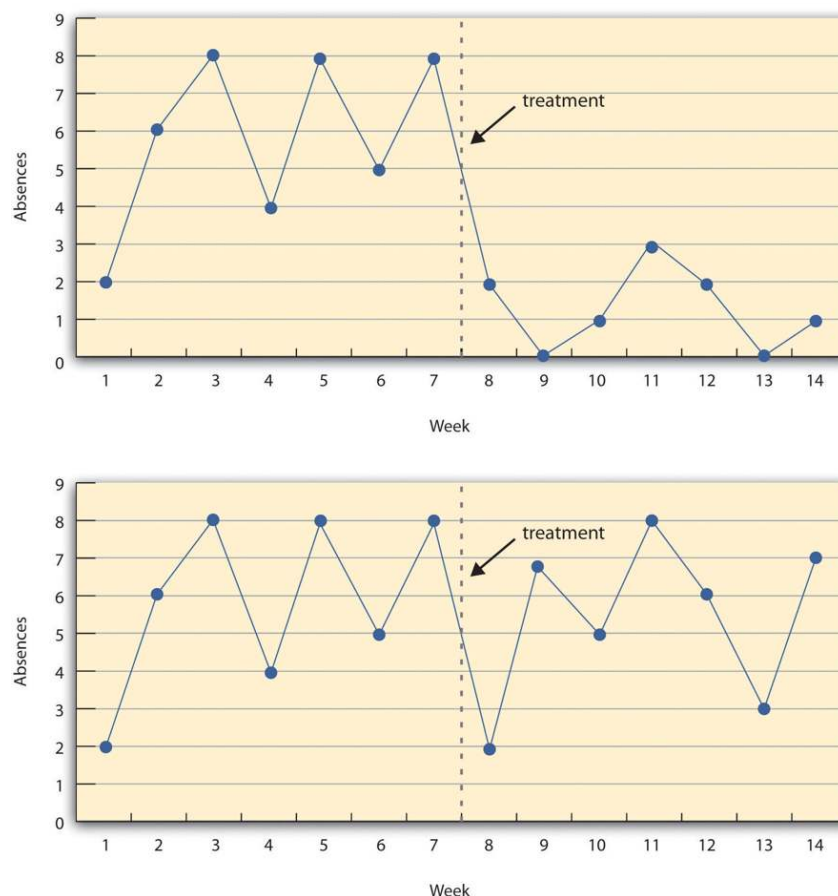
Figure 8.2.1: A Hypothetical Interrupted Time-Series Design. The top panel shows data that suggest that the treatment caused a reduction in absences. The bottom panel shows data that suggest that it did not.
