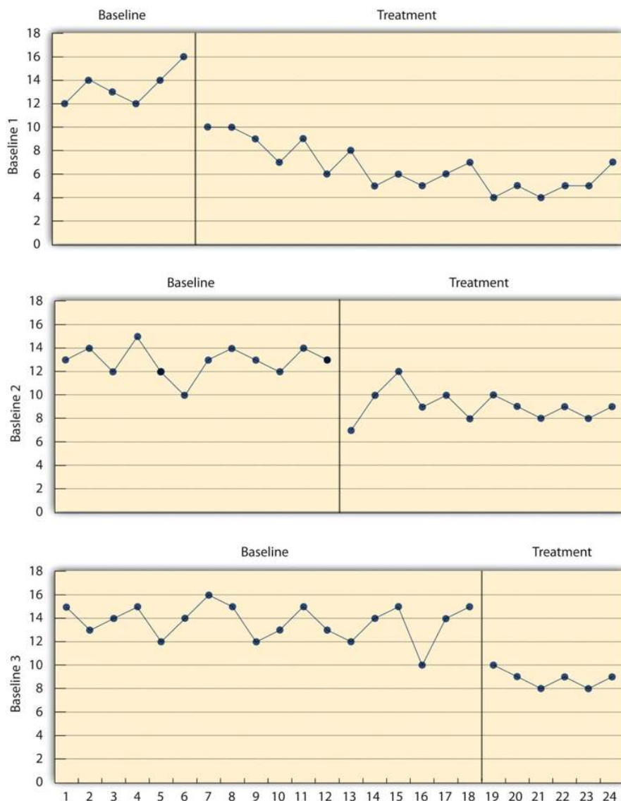
Figure 10.3.3: Results of a Generic Multiple-Baseline Study. The multiple baselines can be for different participants, dependent variables, or settings. The treatment is introduced at a different time on each baseline.
