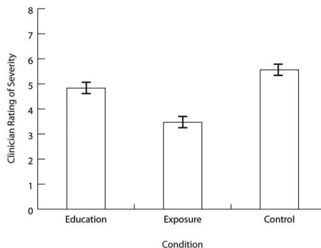
Figure 12.3.1: Mean clinician's rating of phobia severity for participants receiving the education treatment and the exposure treatment. Error bars represent standard errors. Sample APA-Style Bar Graph, With Error Bars Representing the Standard Errors, Based on Research by Ollendick and Colleagues
