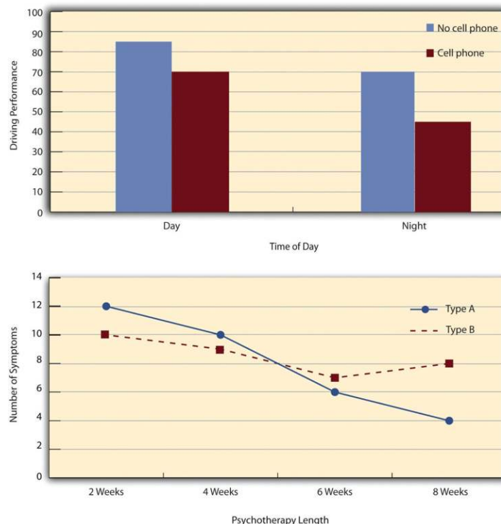
Figure 9.3.1: Two Ways to Plot the Results of a Factorial Experiment With Two Independent Variables
