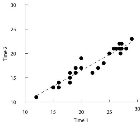
Figure 12.3.3: Sample APA-Style Scatterplot. Relationship between scores on the Rosenberg self-esteem scale taken by 25 research methods students on two occasions one week apart. Pearson's r=0.96 .
