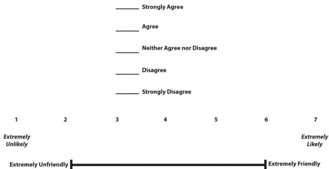
Figure 7.3.2: Example Rating Scales for Closed-Ended Questionnaire Items
