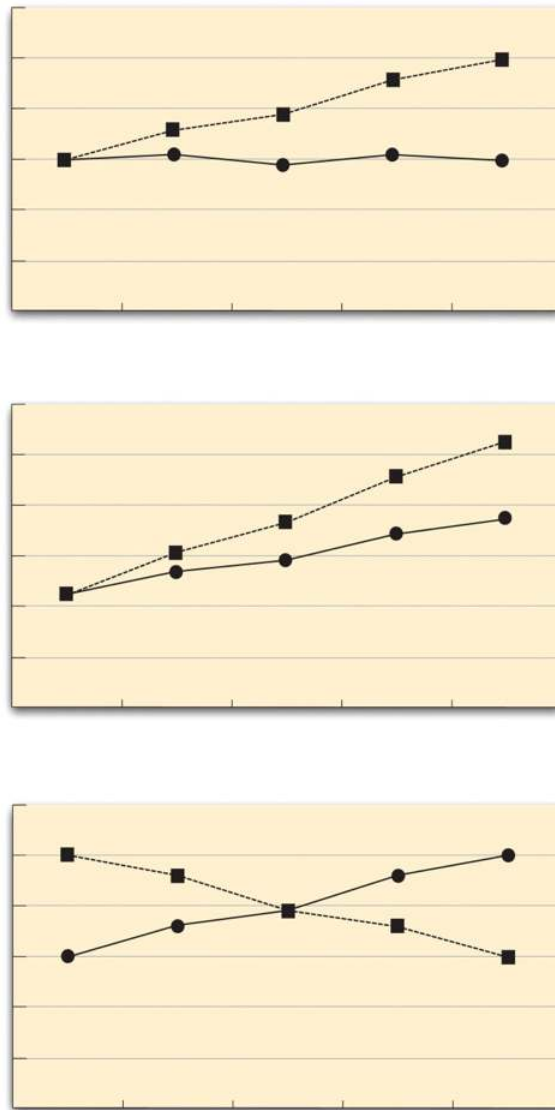
Figure 9.3.3: Line Graphs Showing Different Types of Interactions. In the top panel, one independent variable has an effect at one level of the second independent variable but not at the other. In the middle panel, one independent variable has a stronger effect at one level of the second independent variable than at the other. In the bottom panel, one independent variable has the opposite effect at one level of the second independent variable than at the other.
