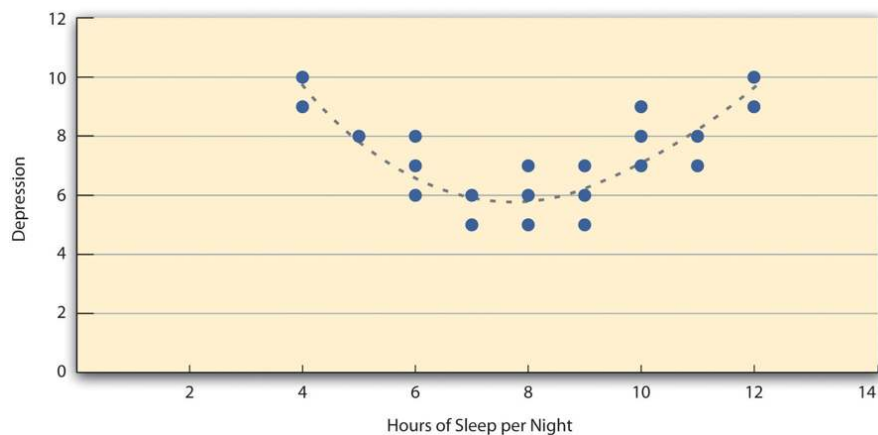
Figure 6.3.4: Hypothetical Nonlinear Relationship Between Sleep and Depression
