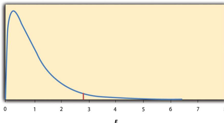
Figure 13.3.2: Distribution of the F Ratio With 2 and 37 Degrees of Freedom When the Null Hypothesis Is True. The red vertical line represents the critical value when \alpha is .05.
