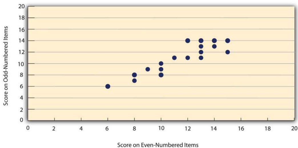
Figure 4.3.2: Split-Half Correlation Between Several College Students' Scores on the Even-Numbered Items and Their Scores on the Odd-Numbered Items of the Rosenberg Self-Esteem Scale
