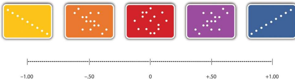
Figure 6.3.3: Range of Pearson's r , From -1.00 (Strongest Possible Negative Relationship), Through 0 (No Relationship), to +1.00 (Strongest Possible Positive Relationship)
