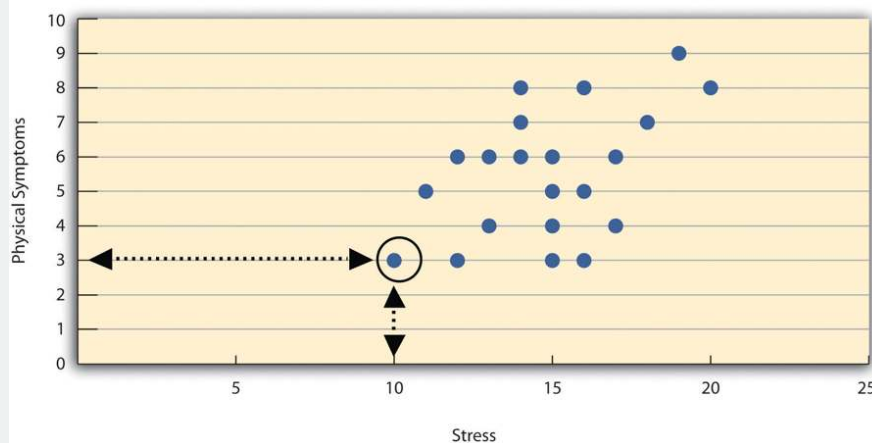
Figure 6.3.2: Scatterplot Showing a Hypothetical Positive Relationship Between Stress and Number of Physical Symptoms. The circled point represents a person whose stress score was 10 and who had three physical symptoms. Pearson's r for these data is +.51 .
