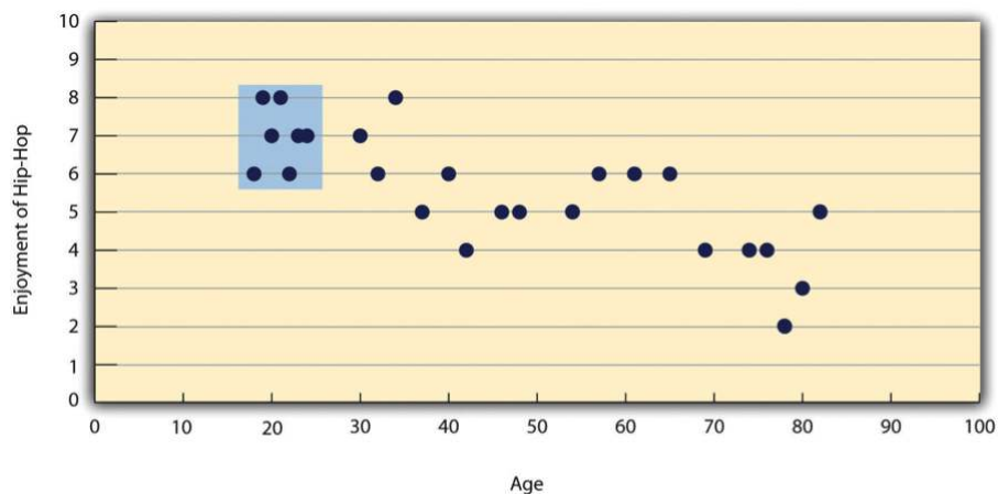
Figure 6.3.5: Hypothetical Data Showing How a Strong Overall Correlation Can Appear to Be Weak When One Variable Has a Restricted Range. The overall correlation here is -.77 , but the correlation for the 18- to 24-year-olds (in the blue box) is 0.
