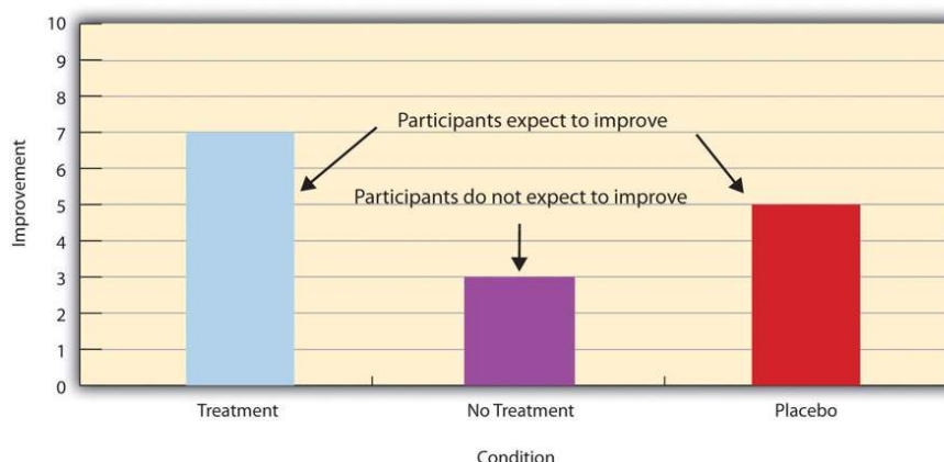
Figure 5.2.2: Hypothetical Results From a Study Including Treatment, No-Treatment, and Placebo Conditions
