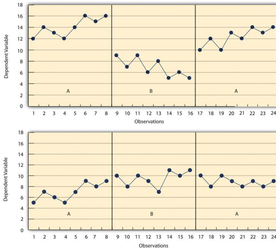
Figure 10.3.4: Results of a Generic Single-Subject Study Illustrating Level, Trend, and Latency. Visual inspection of the data suggests an effective treatment in the top panel but an ineffective treatment in the bottom panel.
