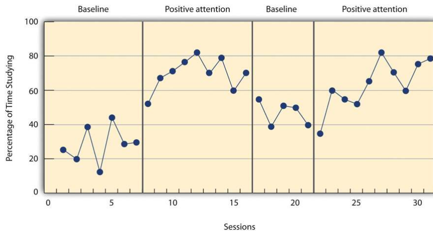
Figure 10.3.2: An Approximation of the Results for Hall and Colleagues' Participant Robbie in Their ABAB Reversal Design
