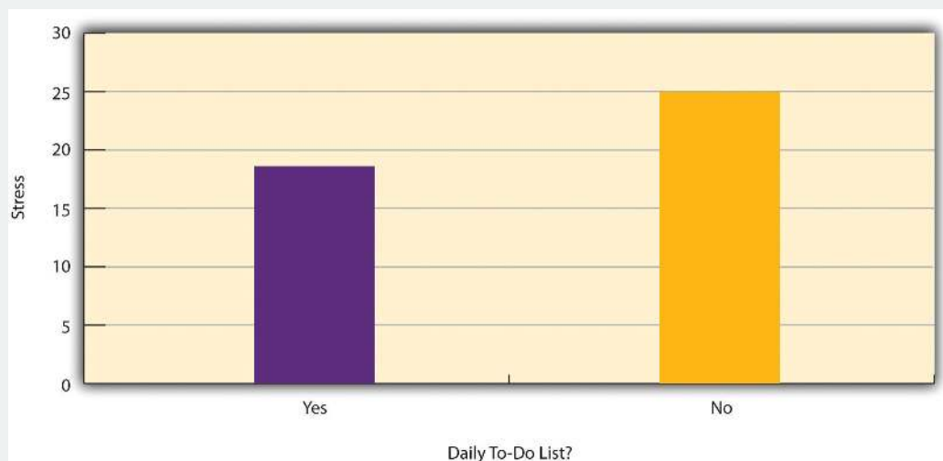
Figure 6.3.1: Results of a Hypothetical Study on Whether People Who Make Daily To-Do Lists Experience Less Stress Than People Who Do Not Make Such Lists
