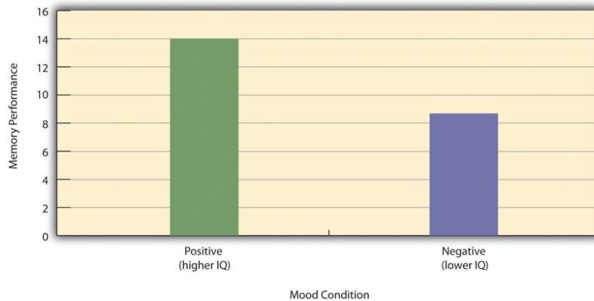
Figure 5.2.1: Hypothetical Results From a Study on the Effect of Mood on Memory. Because IQ also differs across conditions, it is a confounding variable.
