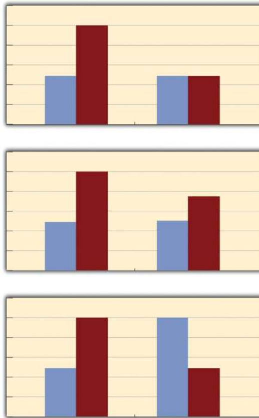
Figure 9.3.2: Bar Graphs Showing Three Types of Interactions. In the top panel, one independent variable has an effect at one level of the second independent variable but not at the other. In the middle panel, one independent variable has a stronger effect at one level of the second independent variable than at the other. In the bottom panel, one independent variable has the opposite effect at one level of the second independent variable than at the other.
