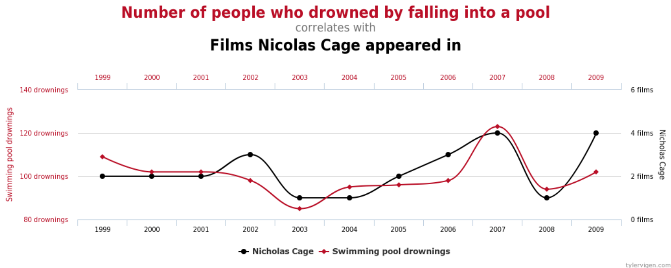
Figure 6.3.6: Example of a Spurious Correlation. Source: http://tylervigen.com/spurious-correlations (CC-BY 4.0)
