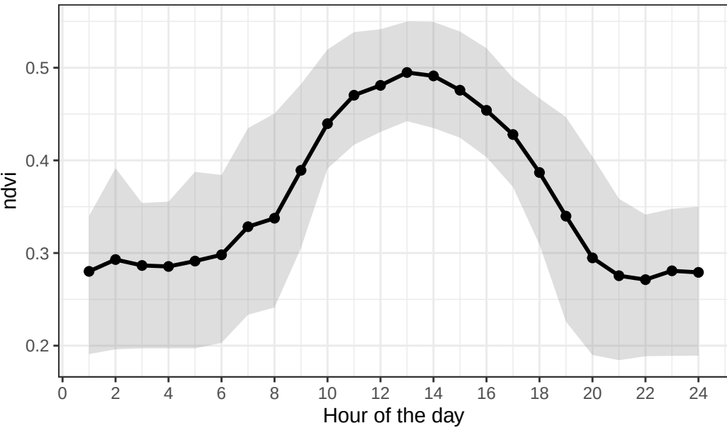
Hourly ndvi
