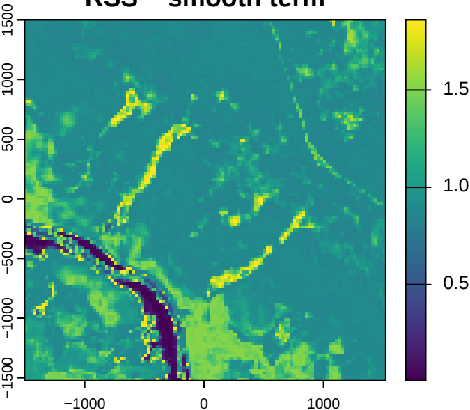
RSS - smooth term
