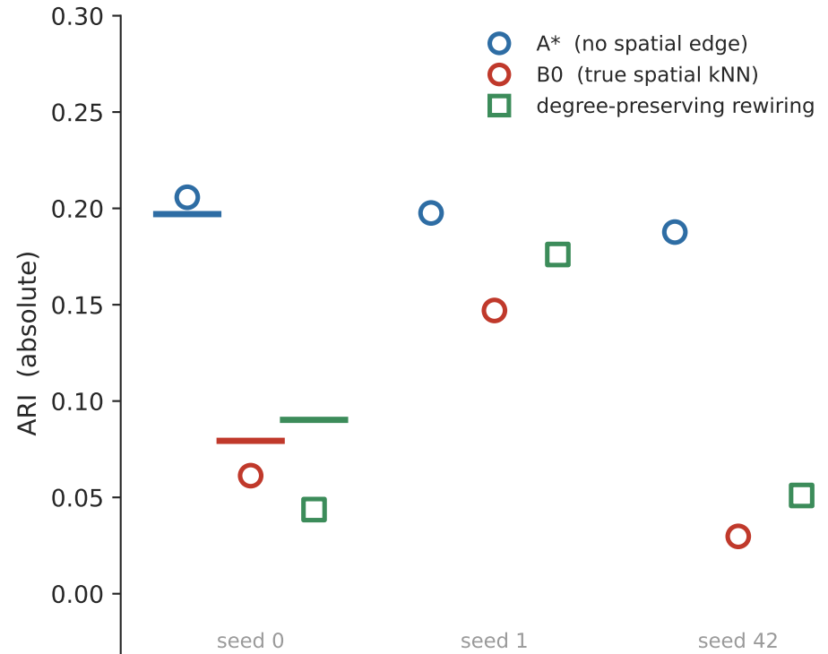
b True spatial graph \approx random graph
