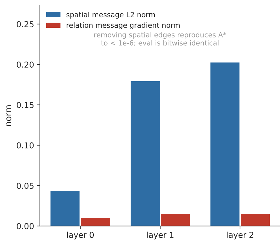
c The relation is live, not missing
