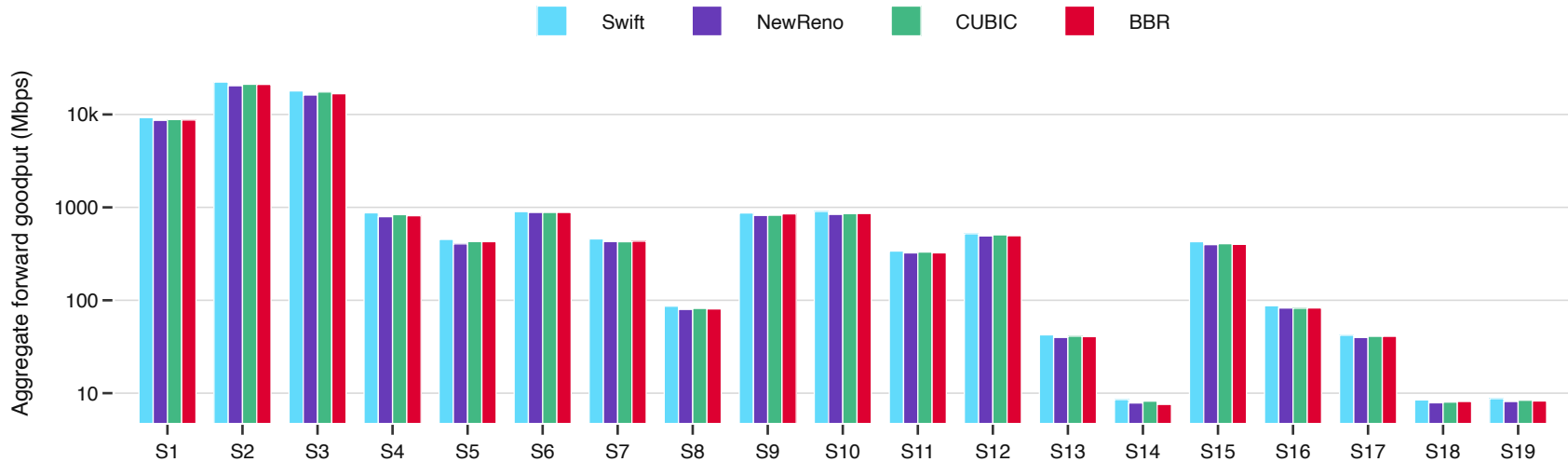
Forward goodput across 19 selected scenarios (TCP-only)
