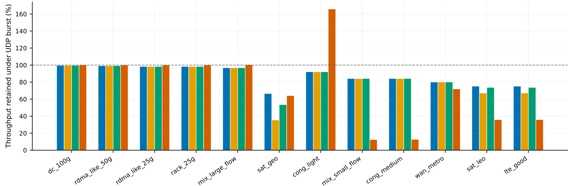
Lark NewReno CUBIC BBR Cross-traffic robustness: throughput retention
