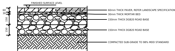
P2-B PAVER TYPE 2 - ON GRADE SCALE 1:10
