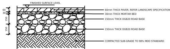
P1-B PAVER TYPE 1 - ON GRADE SCALE 1:10
