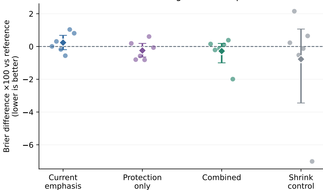
Conditional · Retaining valid older predictions
