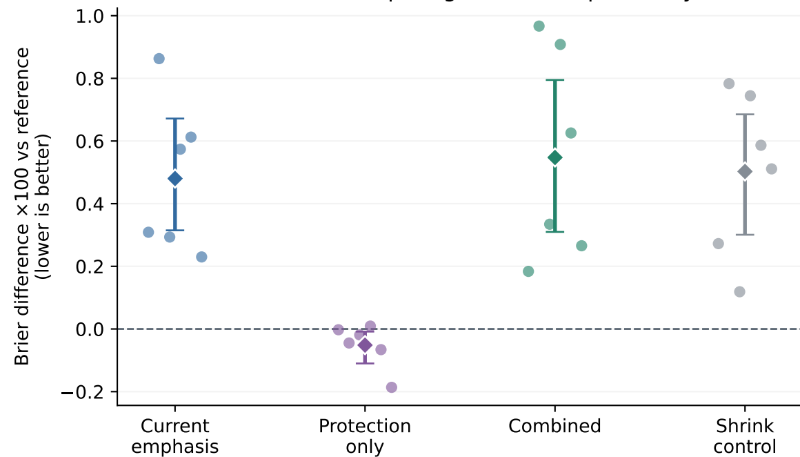
Recurrent · Retaining valid older predictions
