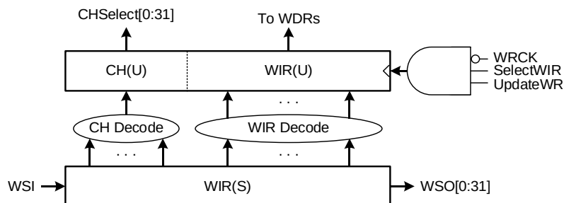
Figure 111 — WIR Channel Select Logic Diagram
