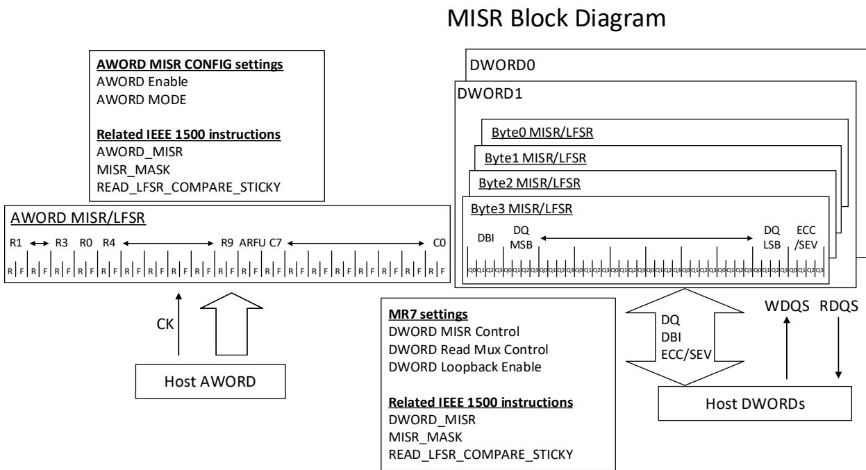
Figure 71 — MISR Features Block Diagram of HBM4
