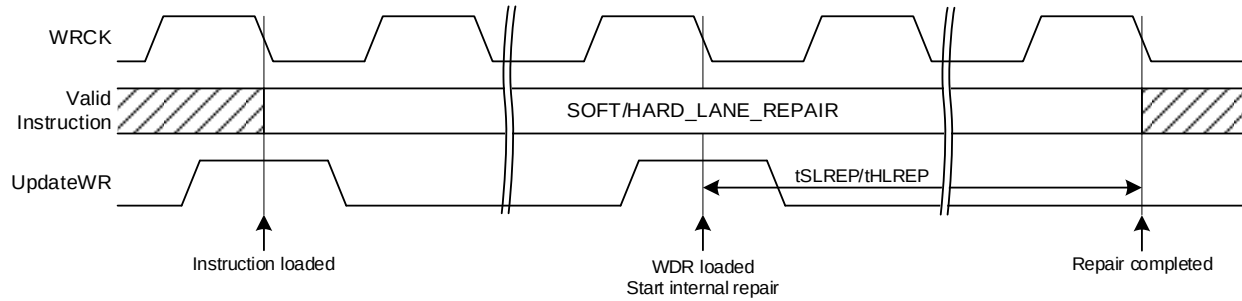
Figure 121 — IEEE1500 Soft_Lane_Repair and Hard_Lane_Repair Instruction Related Timings
