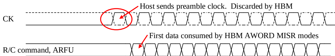
Figure 73 — AWORD MISR Modes Preamble Clock Filter Behavior
