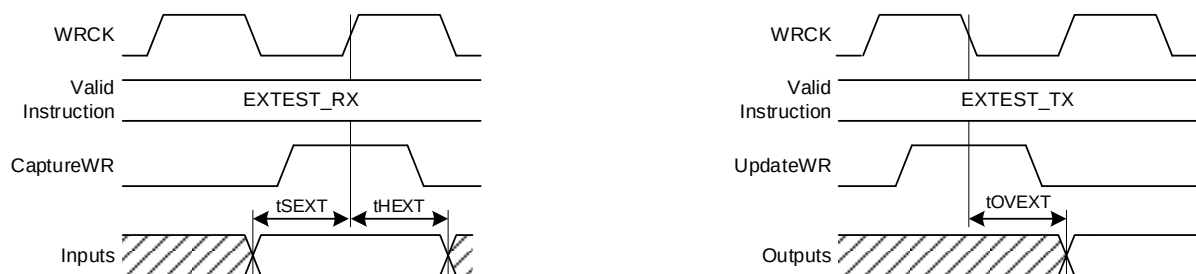
Figure 119 — IEEE1500 EXTEST_RX and EXTEST_TX Instruction Related Timings
