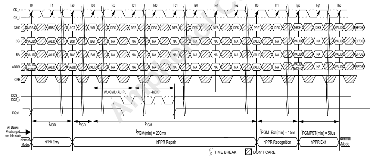
Figure 186 — Hard Fail Row Repair (WR Case)
