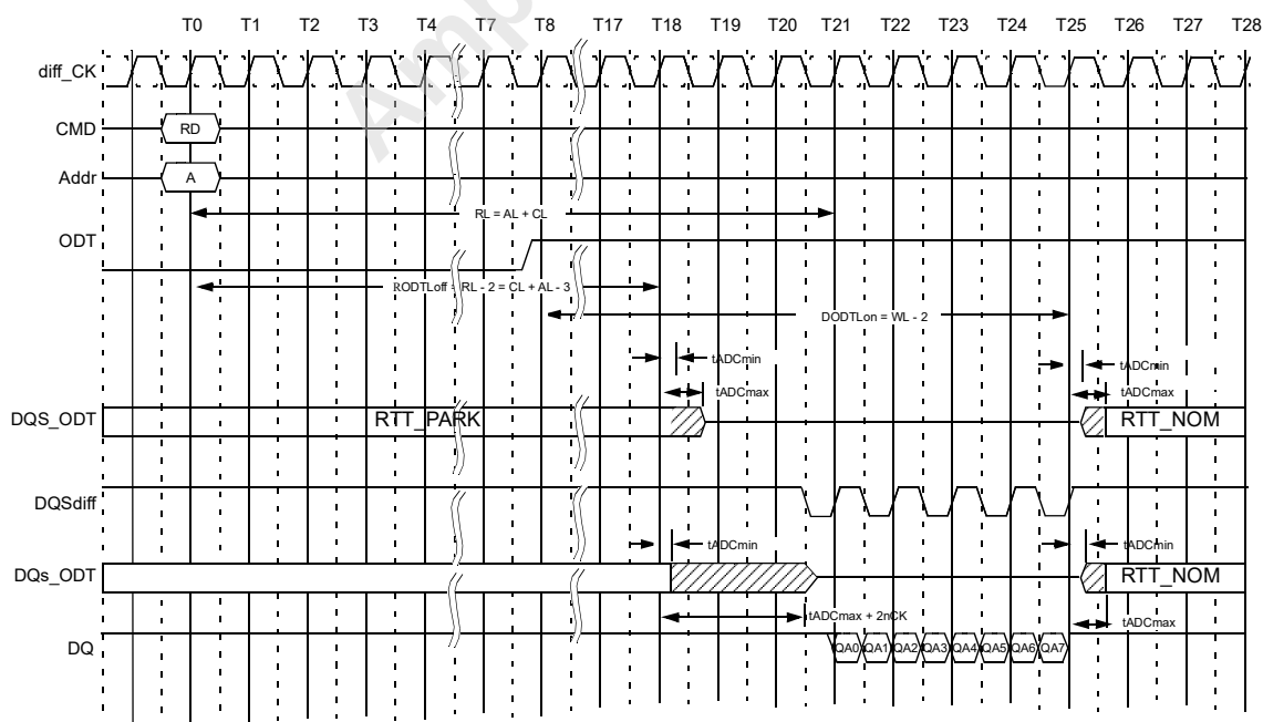
Figure 194 — Example: CL=11, PL=0; AL=CL-1=10; RL=AL+PL+CL=21; CWL=9; DODTLon=AL+CWL-2=17; DODTLoft=AL+CWL-2=17;2tCK preamble)
