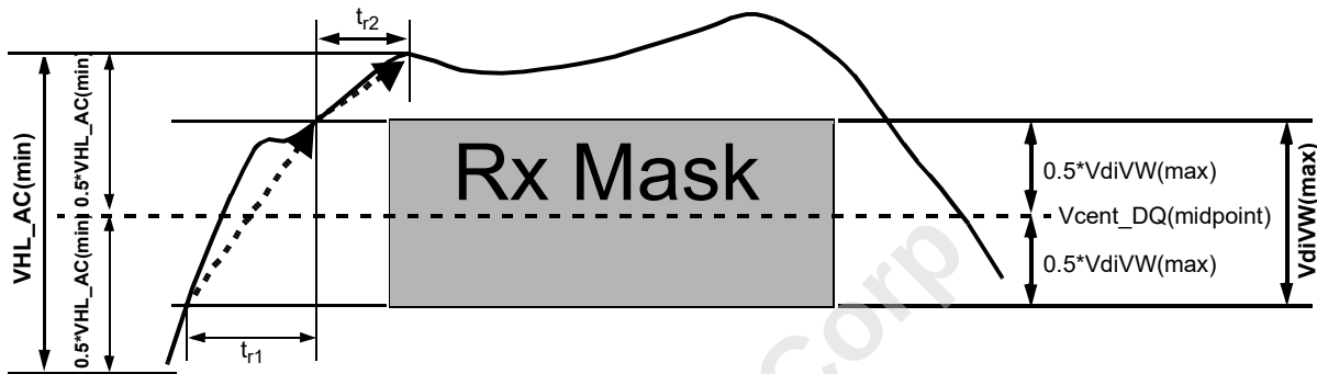
Figure 231 — Slew Rate Conditions For Rising Transition
