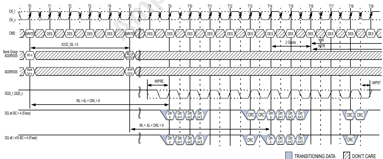
Figure 152 — Consecutive WRITE (BL8/BC4)OTF with 1tCK Preamble and Write CRC in Same or Different Bank Group
