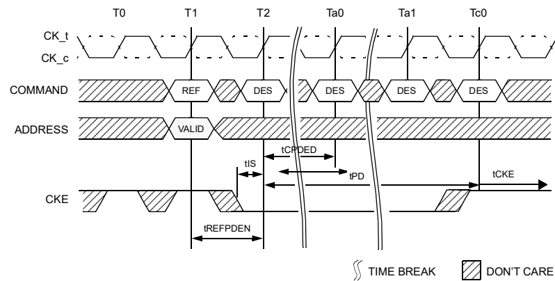
Figure 168 — Refresh Command to Power-Down Entry
