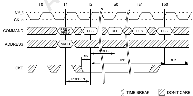
Figure 170 — Precharge/Precharge all Command to Power-Down Entry
