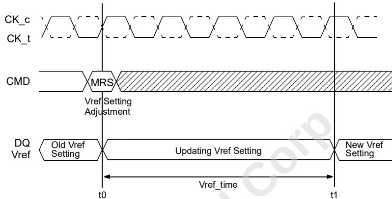
Figure 30 — Vref_time timing diagram
