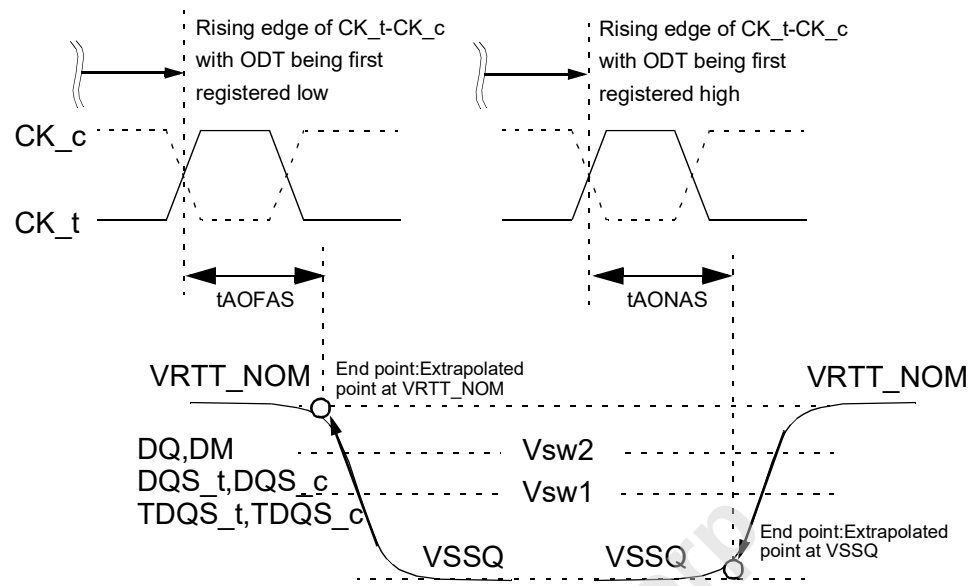
Figure 203 — Definition of tAOFAS and tAONAS
