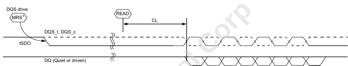
Figure 80 — Read Preamble Training
