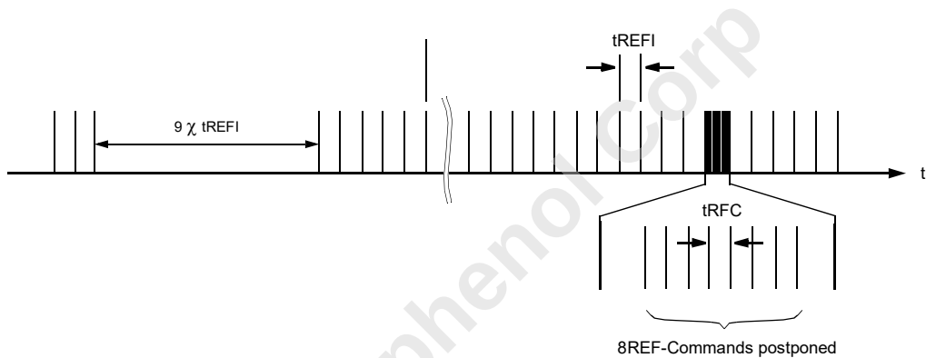
Figure 158 — Postponing Refresh Commands (Example of 1X Refresh mode)
