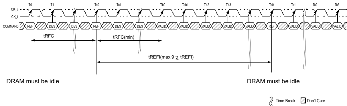
Figure 157 — Refresh Command Timing (Example of 1x Refresh mode)
