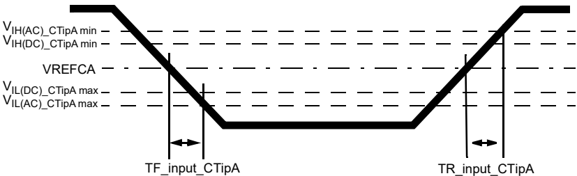
Figure 180 — CS_n and Input A Slew Rate Definition
