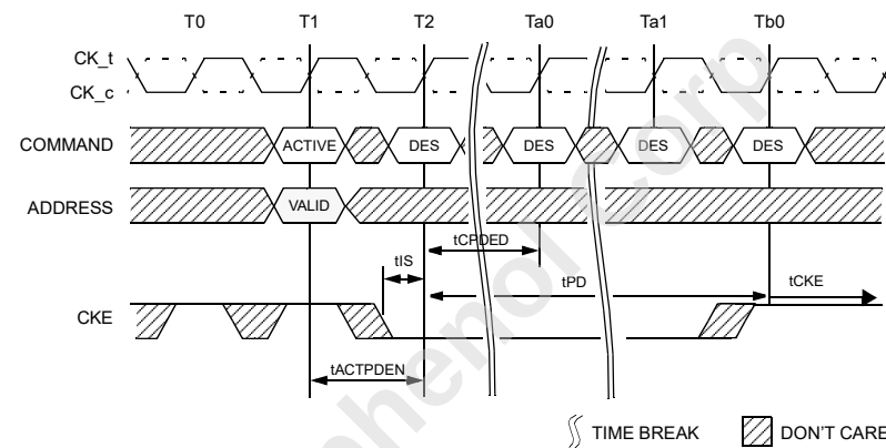
Figure 169 — Activate Command to Power-Down Entry
