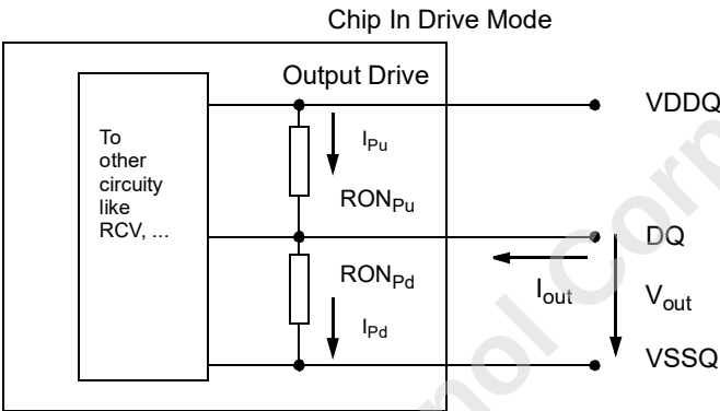
Figure 218 — Output driver
