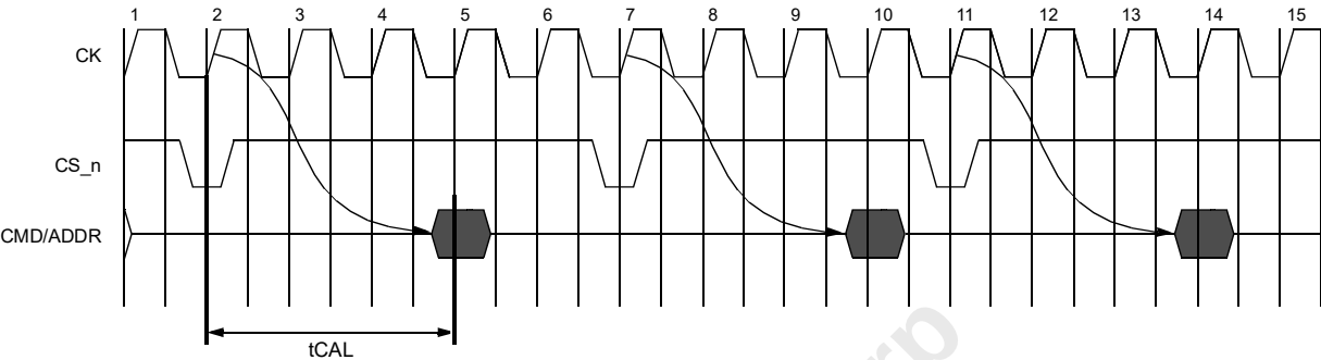
Figure 39 — Definition of CAL
