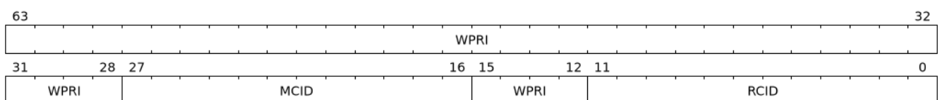
Figure 132. Supervisor Resource Management Configuration ( srmcfg ) register for SXLEN=64
