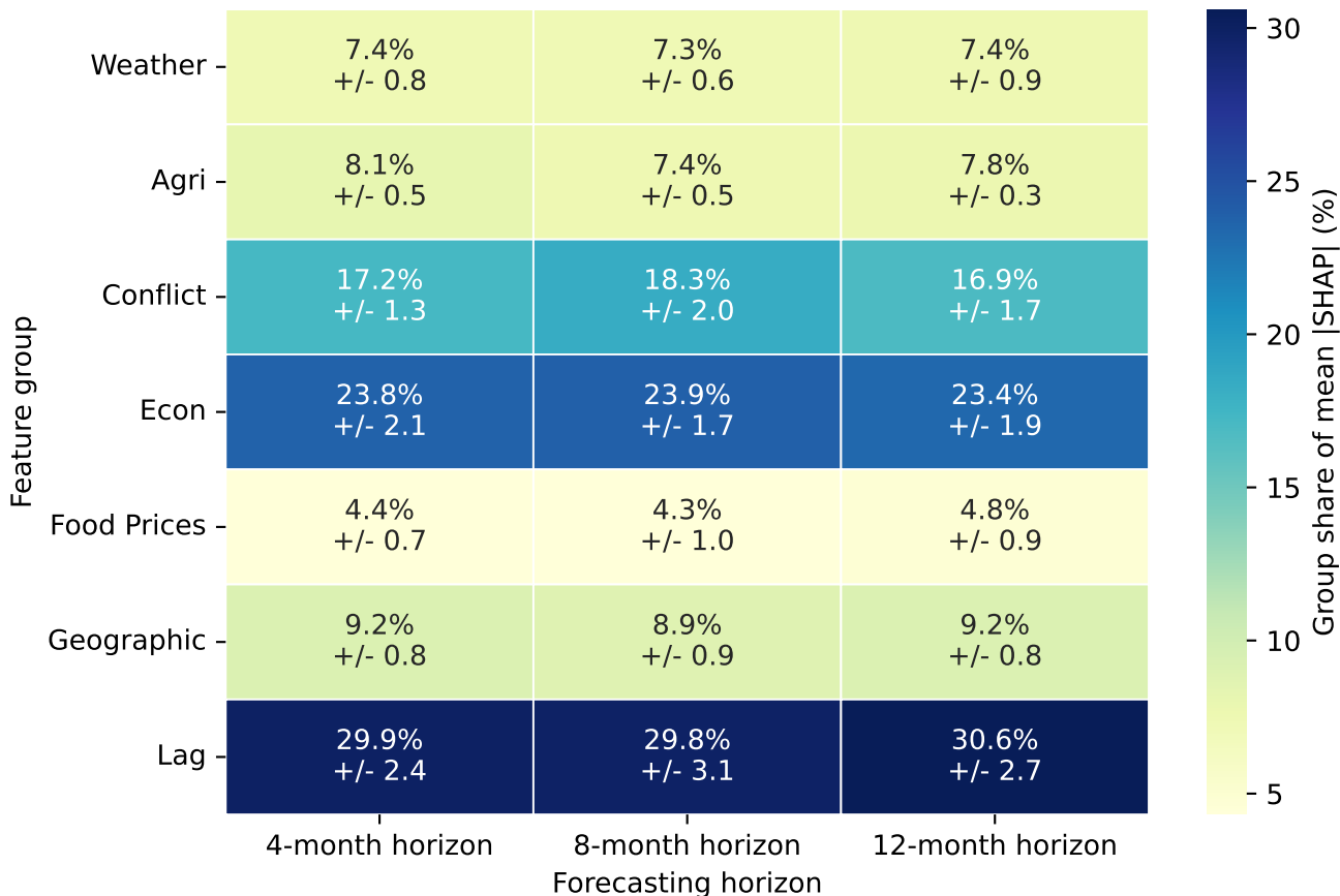
GeoRF Partitioned SHAP Attribution Share
