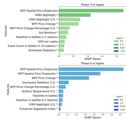
(B) Top 10 Features with Highest SHAP Values for Each Phases in 2nd Layer Nowcasting
