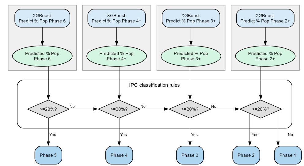
Fig. 3 Ensemble Model Procedure Overview
