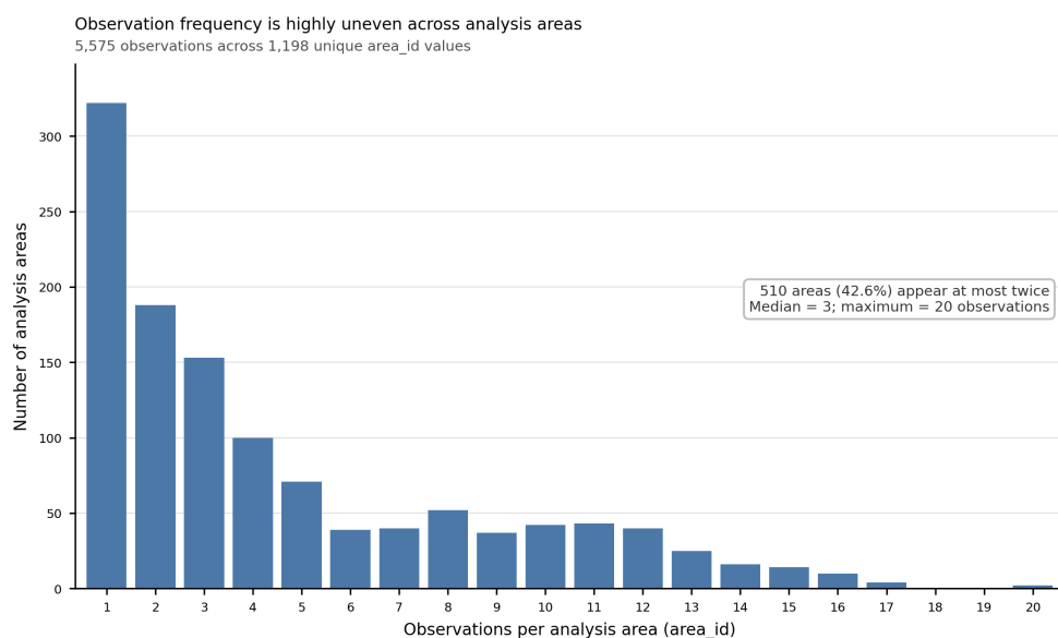
Supplementary Fig. 1 Uneven Observation Frequency Across Analysis Areas
