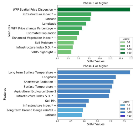
(A) Top 10 Features with Highest SHAP Values for Each Phases in Forecasting
