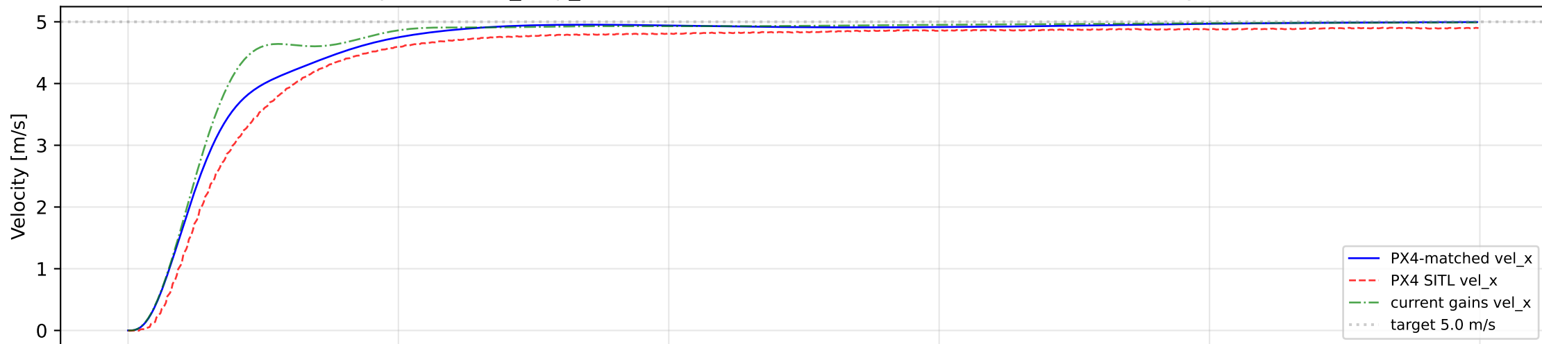
Replicator: vel_step_5 — PX4-matched(blue) vs PX4 SITL (red) vs current (green)
