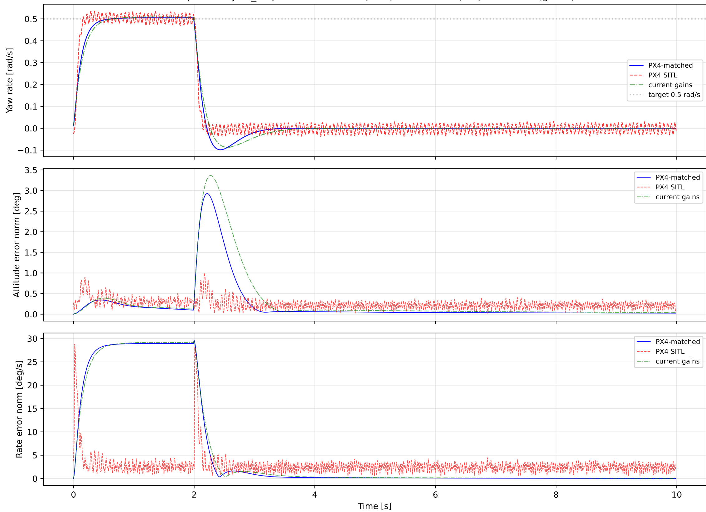
Replicator: yaw_step — PX4-matched (blue) vs PX4 SITL (red) vs current (green)
