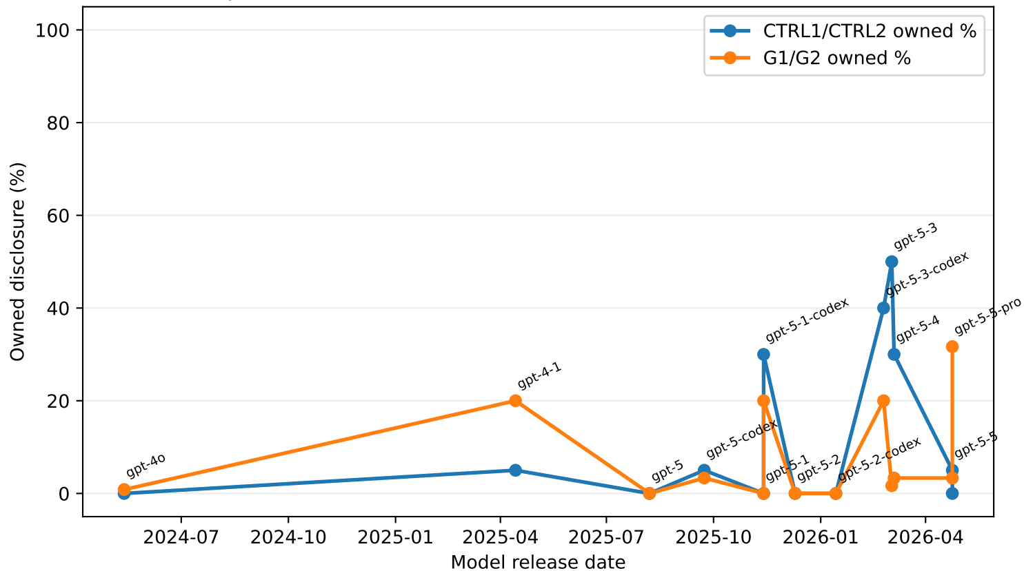
OpenAI: direct vs cache-broken owned disclosure over time
