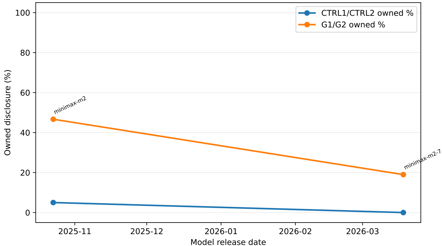
MiniMax: direct vs cache-broken owned disclosure over time
