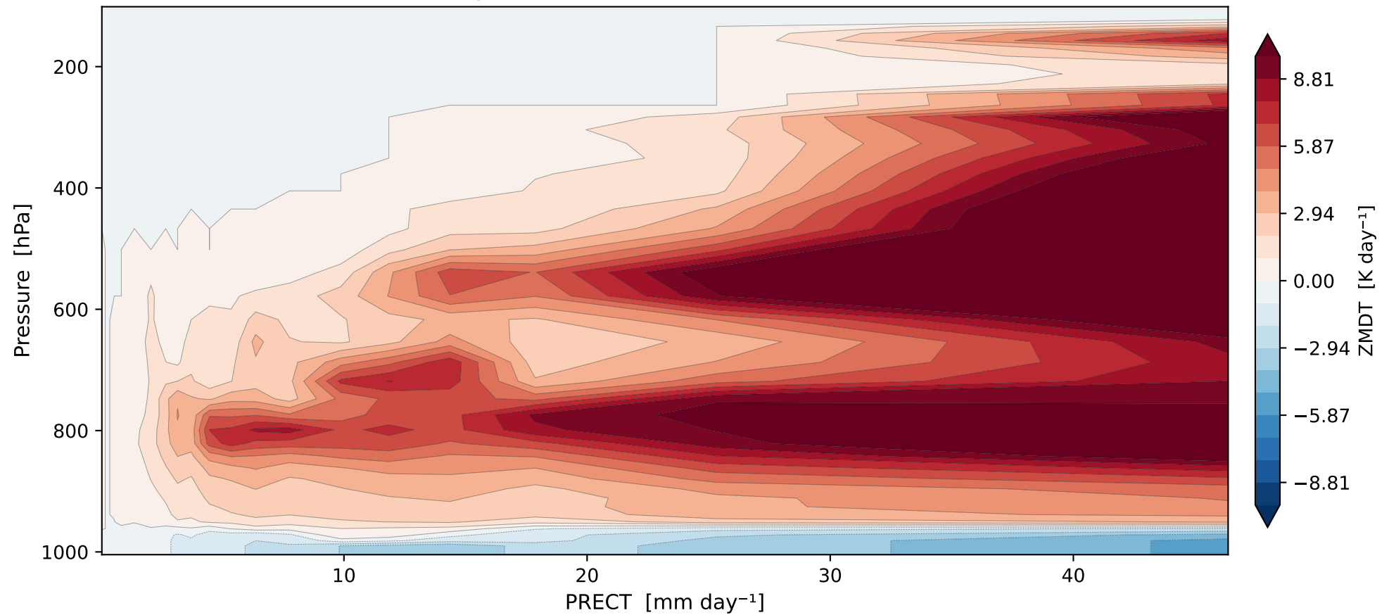
ZMDT sorted by PRECT (20 bins) — TOGA-COARE / CAM7 / L58
