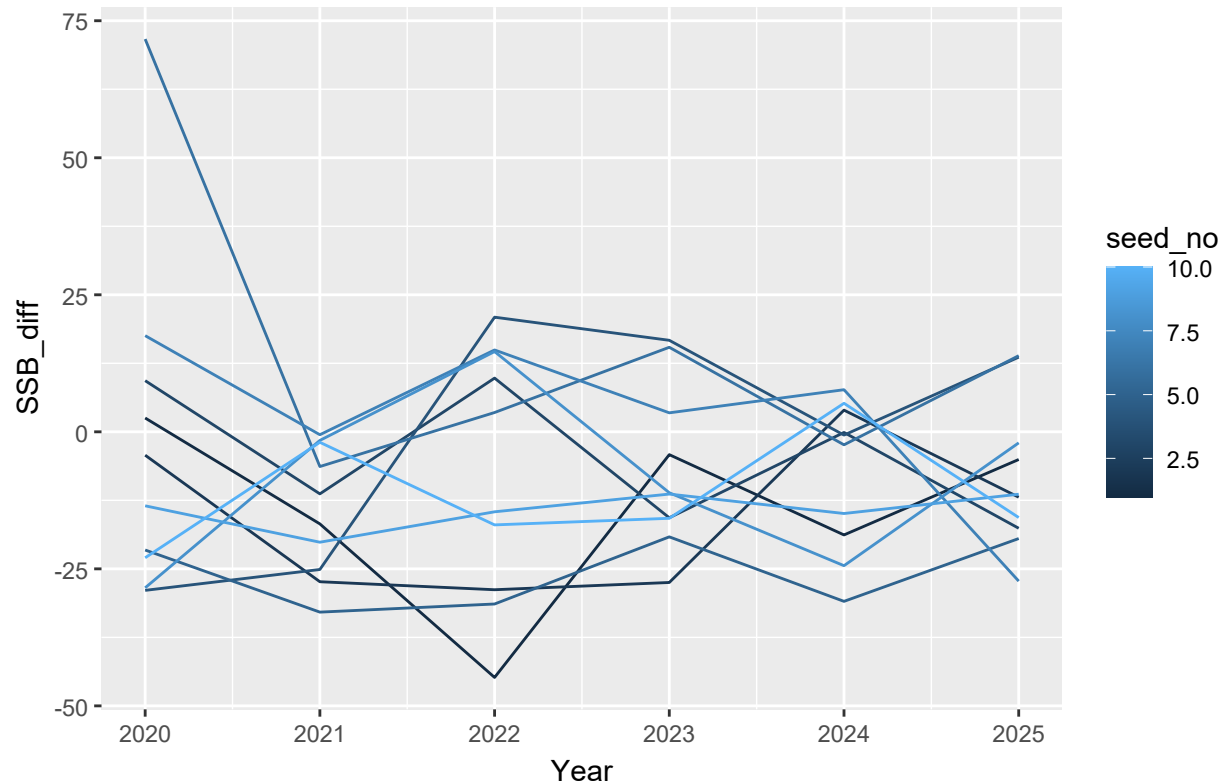
Mod_HistAvgEcov
