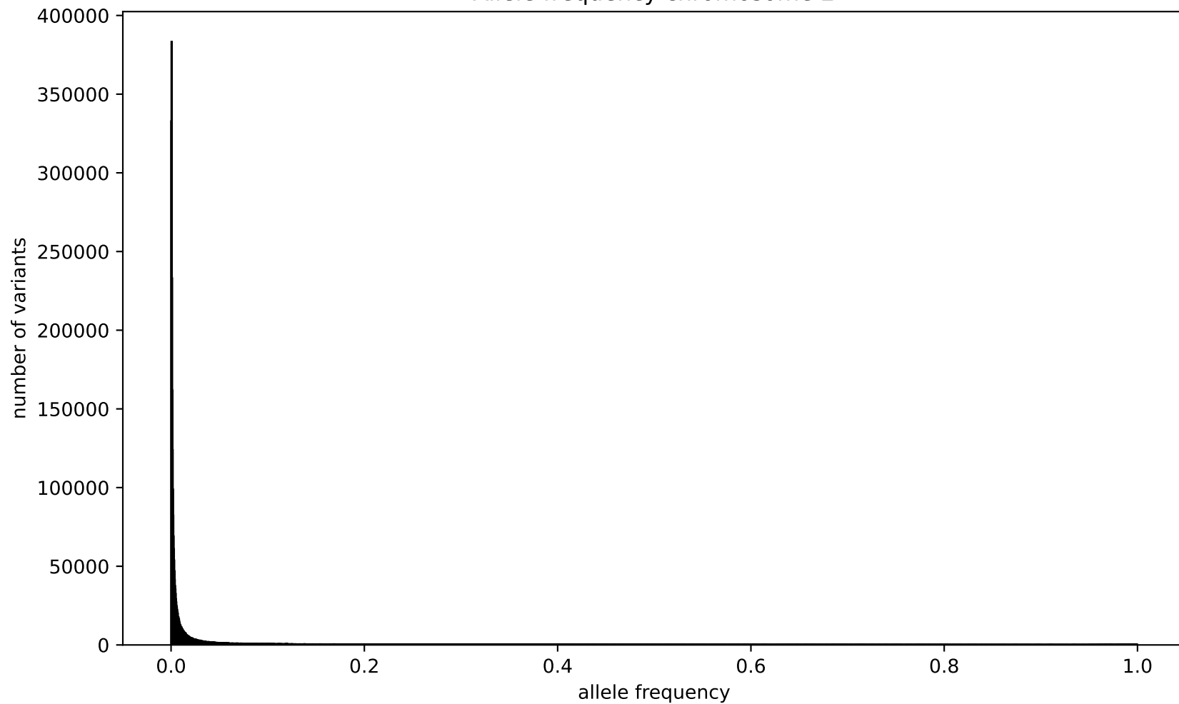
Allele frequency chromosome 2
