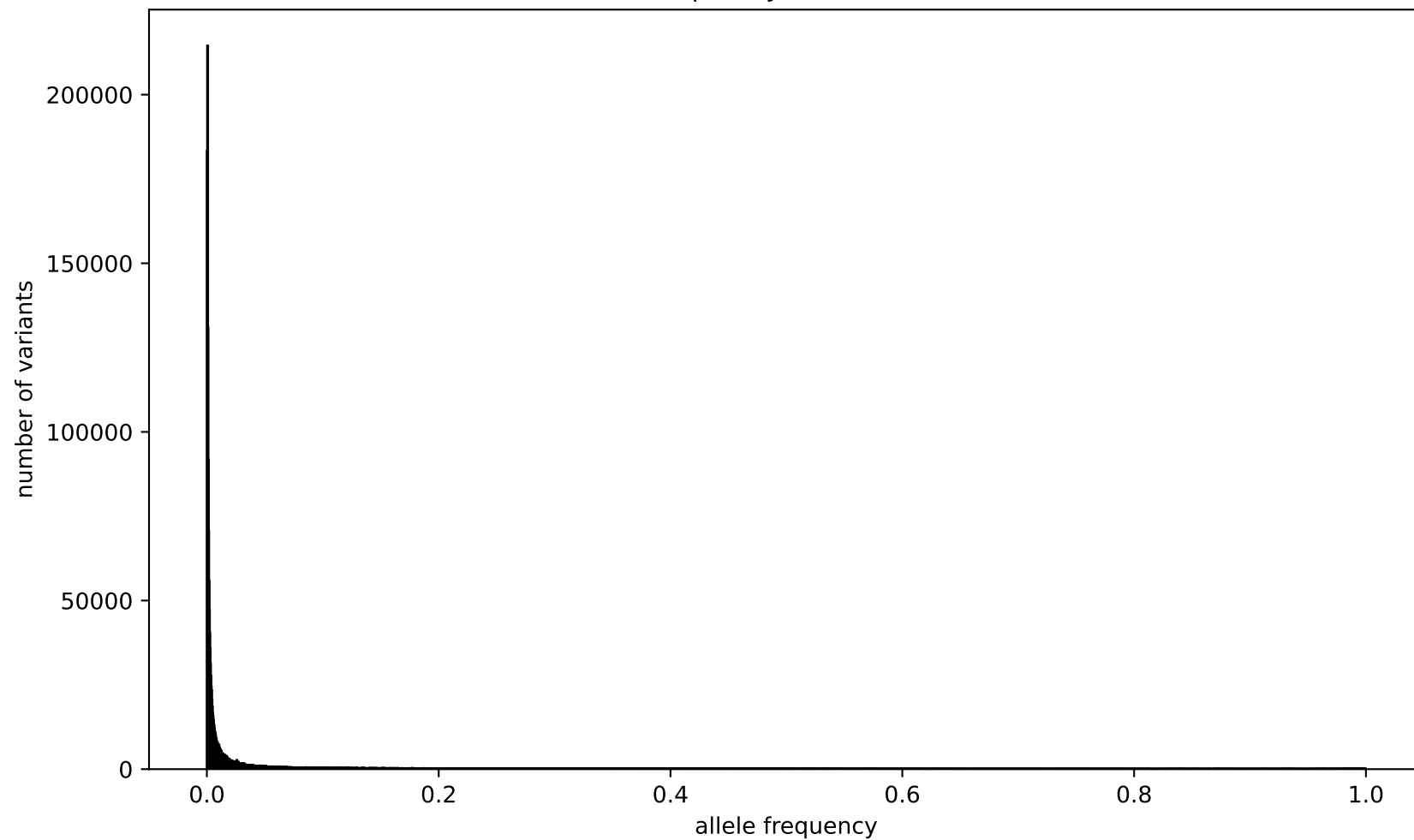
Allele frequency chromosome 10
