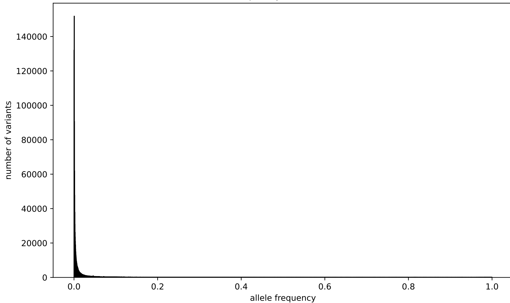
Allele frequency chromosome 16
