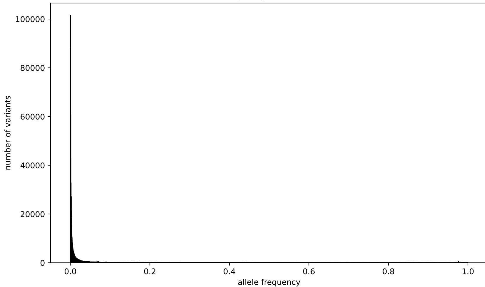
Allele frequency chromosome 19
