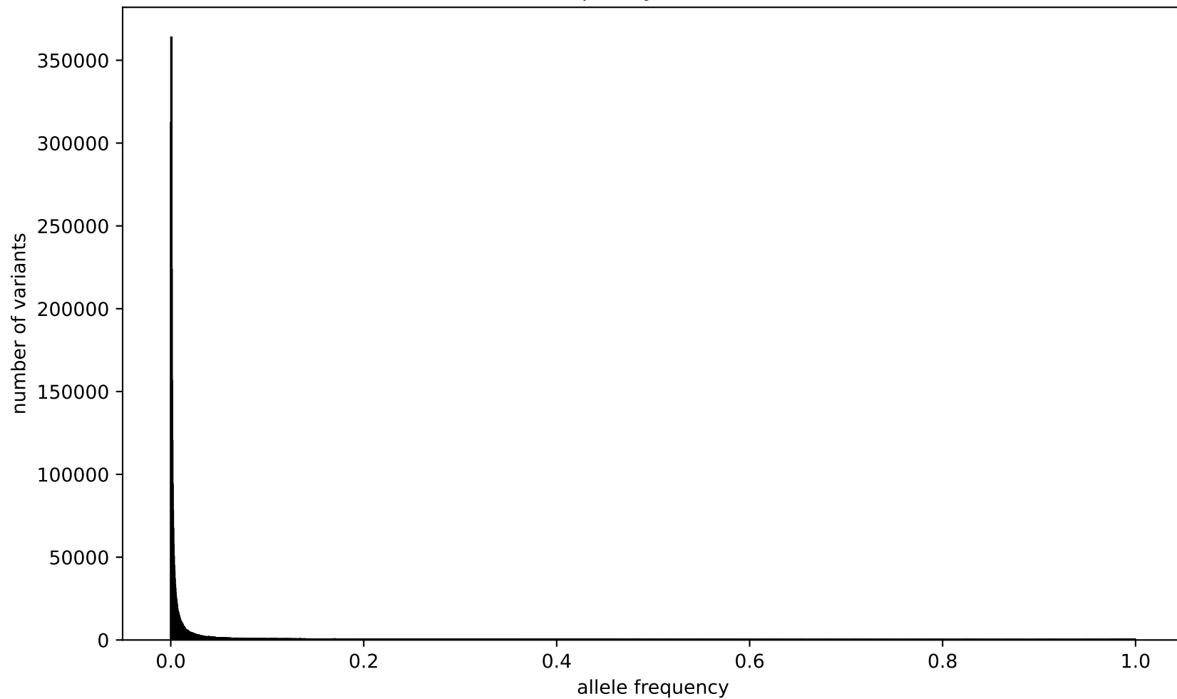
Allele frequency chromosome 1
