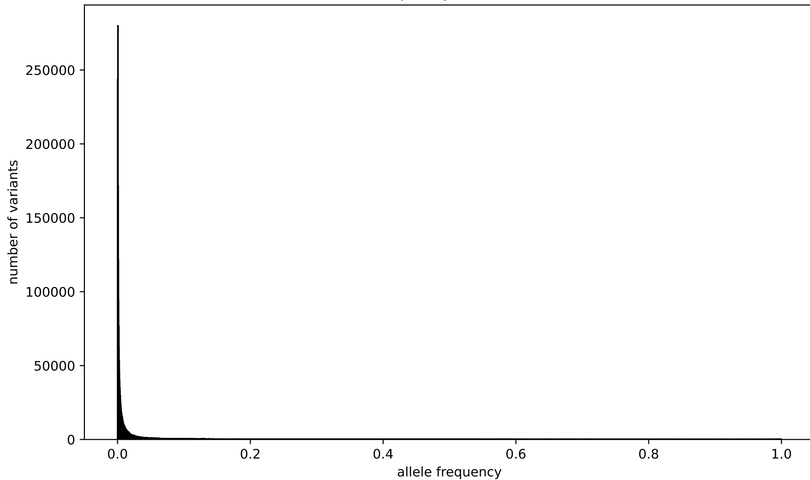
Allele frequency chromosome 5
