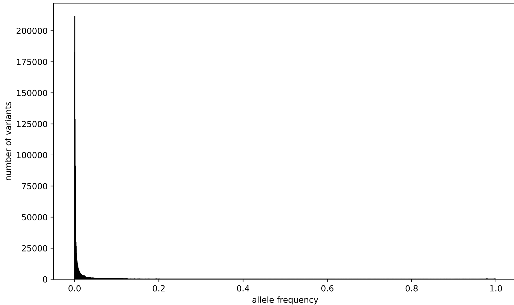
Allele frequency chromosome 11
