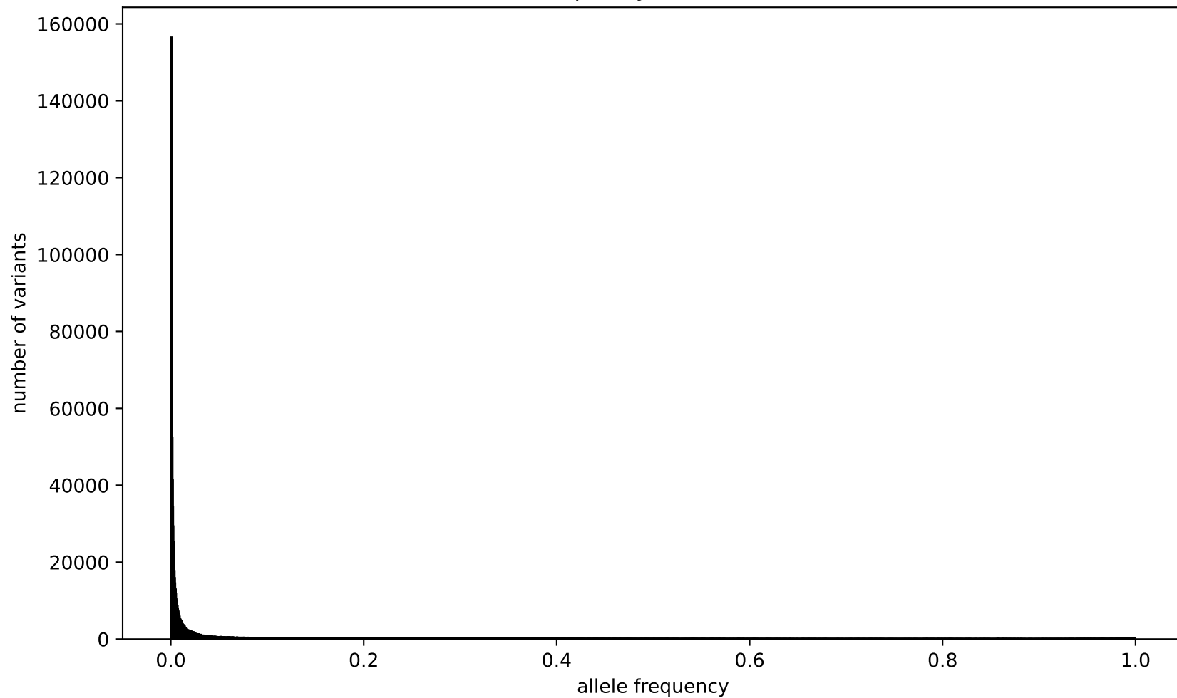
Allele frequency chromosome 13
