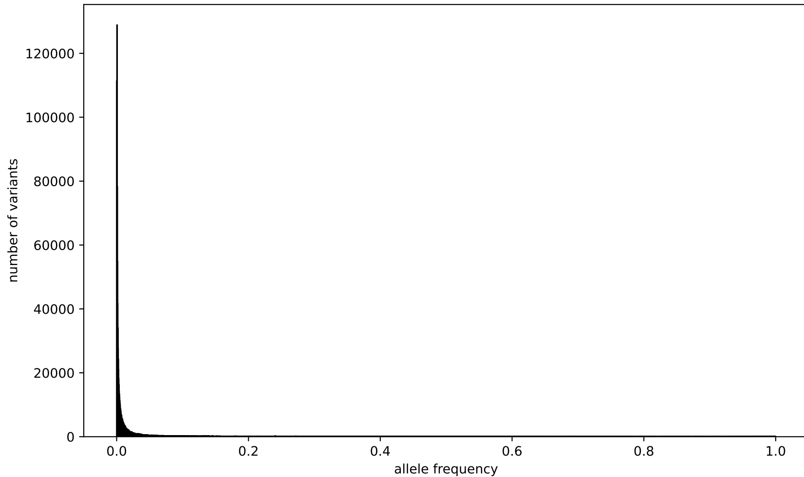
Allele frequency chromosome 15
