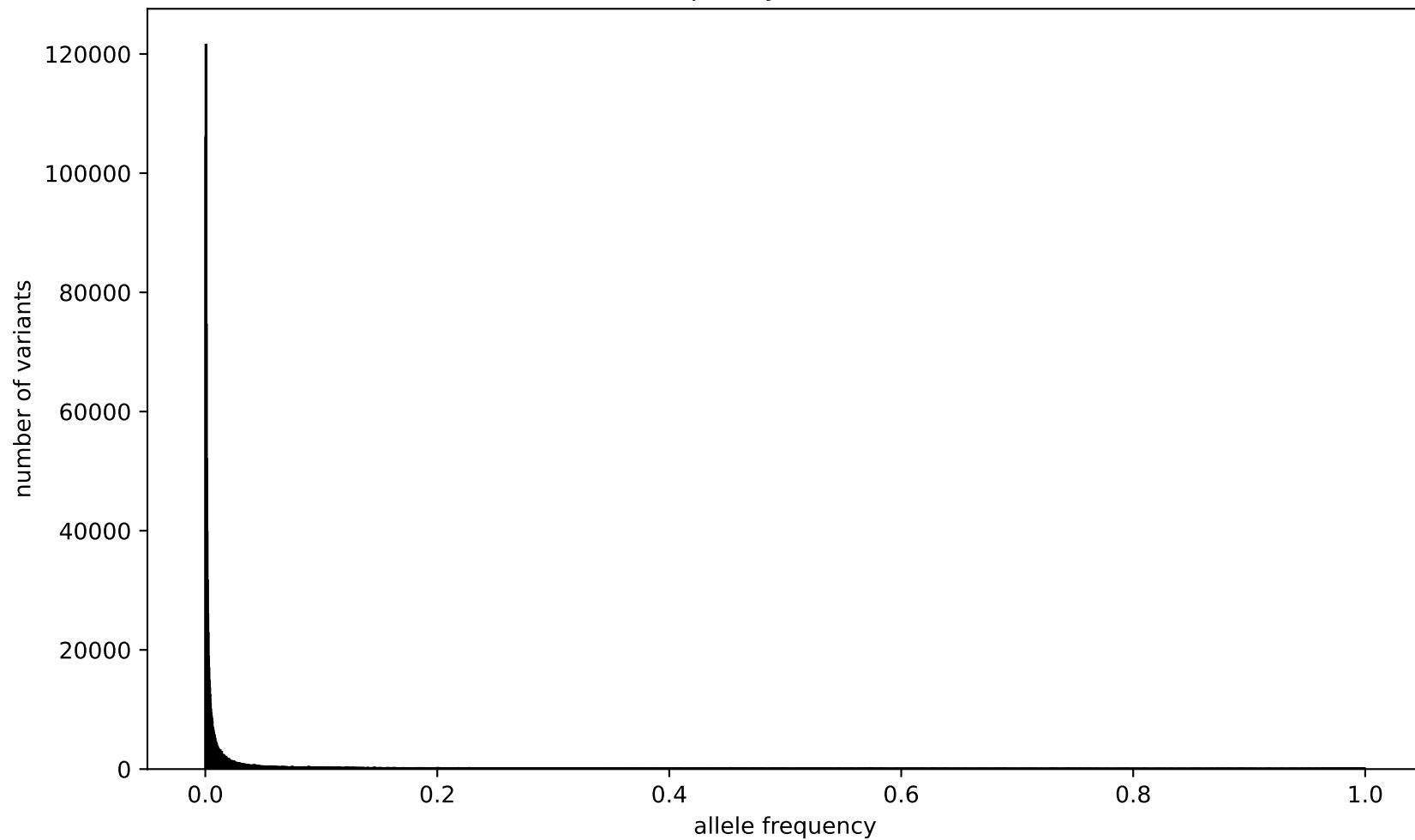
Allele frequency chromosome 18
