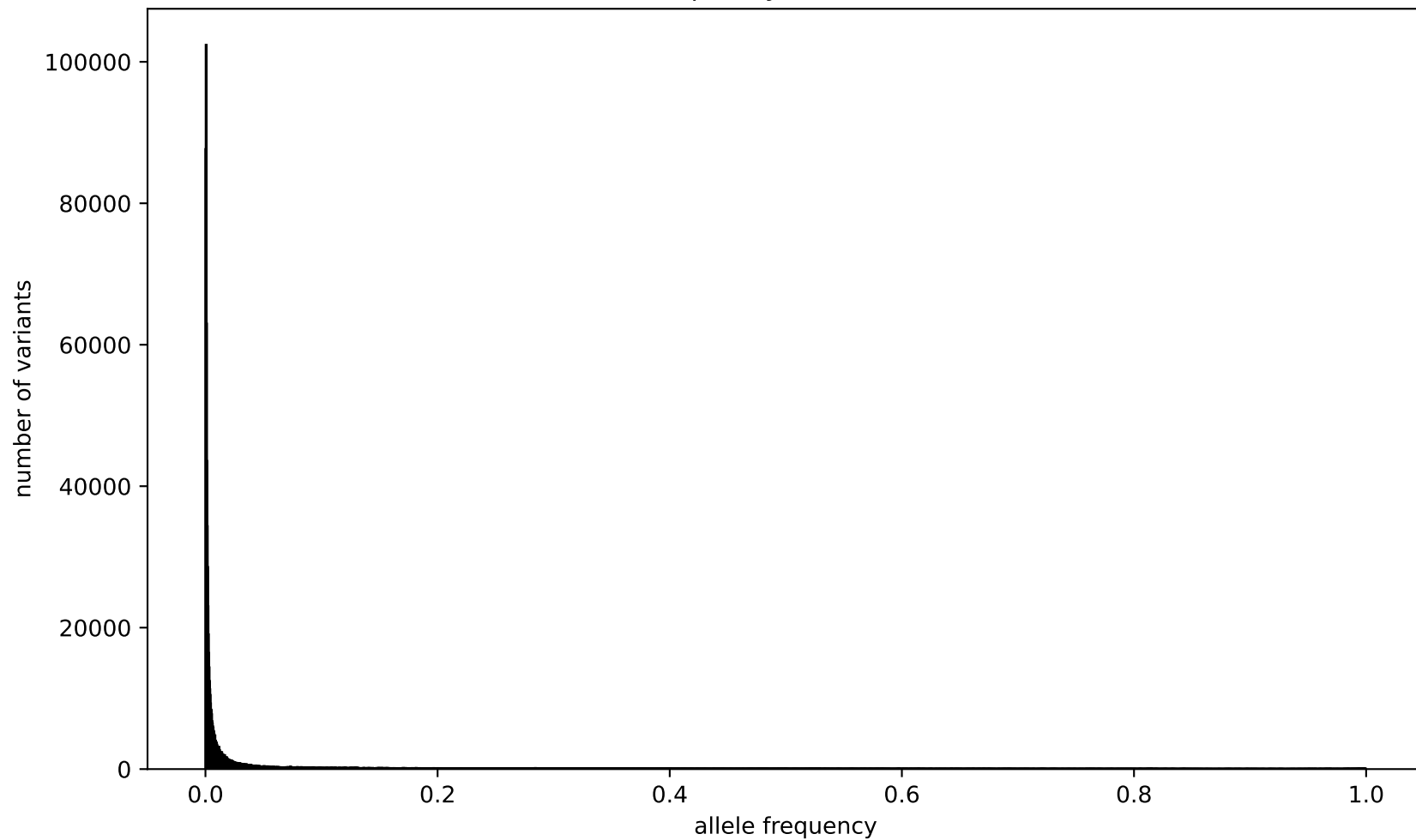
Allele frequency chromosome 20
