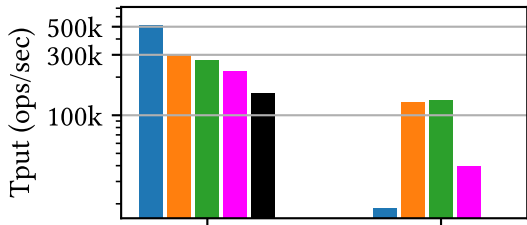
YCSB A
