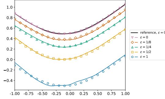
FIG. 9. Profiles of the learned value function v_\theta and of the empirical costs \hat{J}(u_\alpha) for the SOCP in subsection 4.5, with fixed d = 10^4 and varying perturbation parameter \epsilon . Lines depict s \mapsto v_\theta(0, s\mathbf{1}_d) , whereas markers in the corresponding colors depict \hat{J}(u_\alpha) defined in (4.5) with the initial condition \tilde{X}_0^m = s\mathbf{1}_d .
