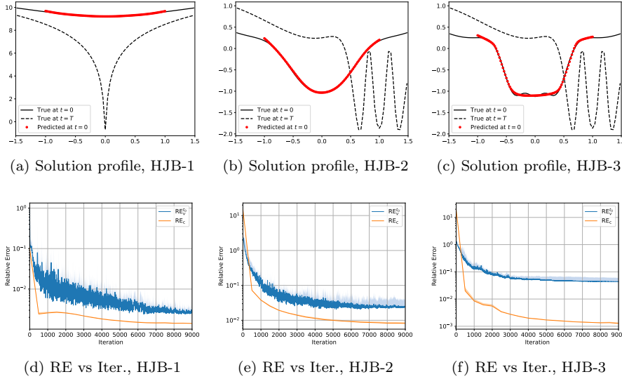
FIG. 2. Results for HJB-1, -2, and -3 in subsection 4.2 with d = 10^4 . Shading denotes the five-run mean plus or minus twice the SD in (a)–(c) and the five-run mean plus twice the SD in (d)–(f). The final-iteration statistics are reported in Table 1.
