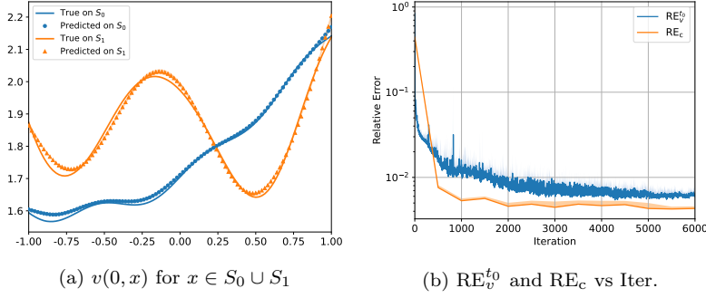
FIG. 5. Results for the complex-dynamics SOCP in subsection 4.3 with d = 10^4 . Shading denotes the five-run mean plus or minus twice the SD in (a) and the five-run mean plus twice the SD in (b).
