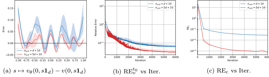
FIG. 3. Results for HJB-3 in subsection 4.2 with d = 2000 and n_{\text{unit}} = d + 10 or n_{\text{unit}} = 5d + 10 . Shading denotes the five-run mean plus or minus twice the SD in (a) and the five-run mean plus twice the SD in (b)–(c). The final-iteration statistics are reported in Table 1.
