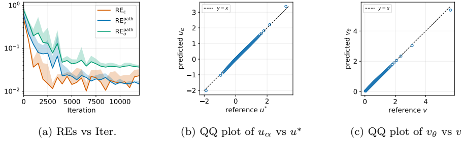
FIG. 8. Results for the SOCP in subsection 4.4 with d = 10^4 . In (a), shading denotes the five-run mean plus twice the SD. In (b) and (c), the quantile-quantile (QQ) plots compare u_\alpha and v_\theta , respectively, evaluated on the points (t_n, \bar{X}_n^m) introduced in (4.5).
