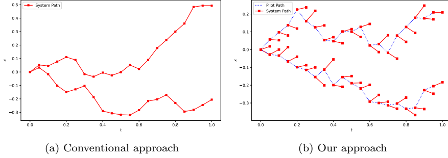
FIG. 1. Comparison of conventional and pilot-system path simulations. The horizontal and vertical axes represent time and state, respectively. In (b), red segments are system-path branches from the pilot path.
