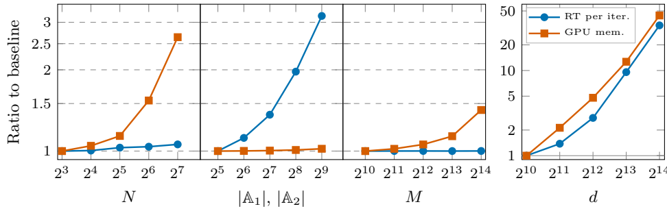
FIG. 7. Relative per-iteration runtime and GPU memory under parameter sweeps around the configuration of subsection 4.3 with d = 10^4 . In each panel, “Ratio to baseline” denotes per-iteration runtime or GPU memory divided by its respective value at the smallest displayed parameter value. Per-iteration values correspond to the outer iteration of Algorithm 3.1, indexed by i . Device: 4 \times A100 .
