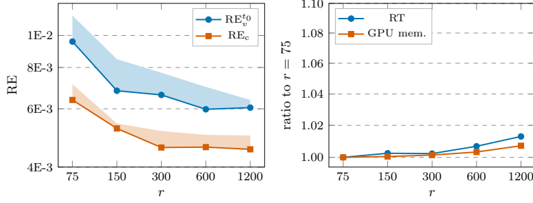
FIG. 6. Sensitivity to the test-function output dimension r for the SOCP example in subsection 4.3 with d = 10^4 . Shading denotes the five-run mean plus twice the SD. Device: 4 \times A100 .
