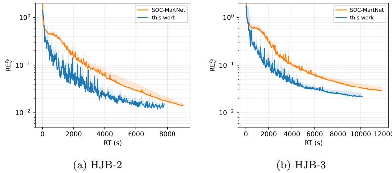
FIG. 4. Relative errors versus the RT for Algorithm 3.1 and SOC-MartNet [16] on HJB-2 and -3 in subsection 4.2 with d = 10^4 . The curves and shading denote the mean and the mean plus twice the SD over the independent runs of each method. Device: 8 \times A100 .
