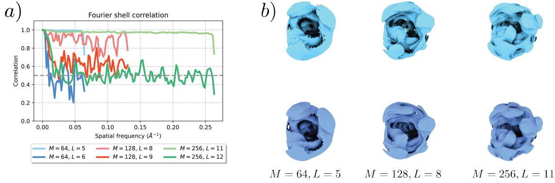
Figure 3.1: Result of running Alg. 1 on the dataset EMD-2660 [59] from the online electron microscopy data bank [34]. (a) FSC curves for the reconstructins, for different values of bandlimit L and image size M . (b) Reconstructions (top) and ground truth structures (bottom).
