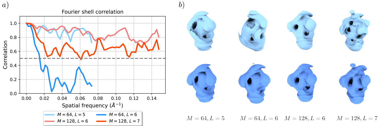
Figure 3.2: Result of running Alg. 1 on the dataset EMD-32743 [27] from the online electron microscopy data bank [34]. (a) FSC curves for the reconstructins, for different values of bandlimit L and image size M . (b) Reconstructions (top) and ground truth structures (bottom).
