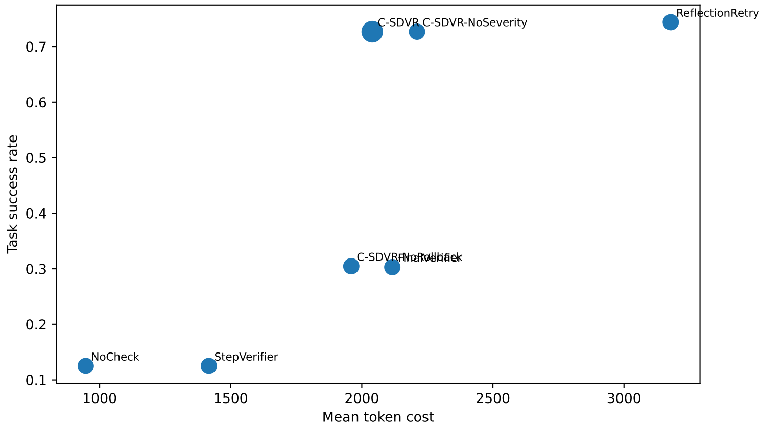
Executable benchmark: success-cost trade-off
