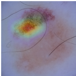
Grad-CAM
