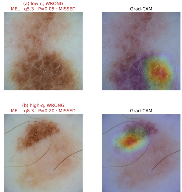
Fig. 2. Grad-CAM on the post-gate feature map. P is P(\text{malignant}) , q the expert quality rating. (a) missed melanoma, low quality, attention off the lesion; (b) missed melanoma, high quality, attention correct. Maps are 7 \times 7 upsampled, indicating approximate attention only.
