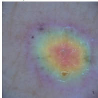
NON-HARD
