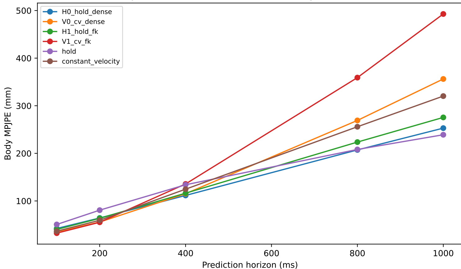
P-only dev rollout; learned models averaged over 3 seeds
