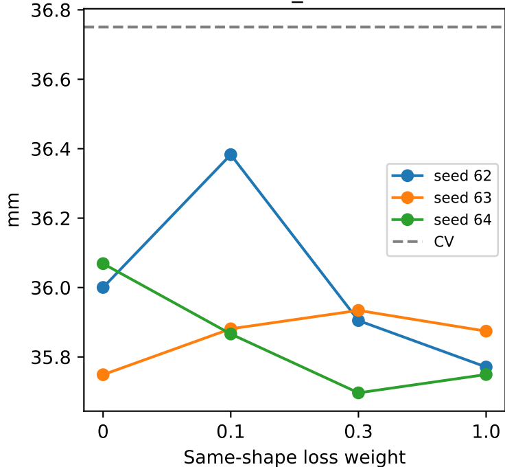
fk22_mm
