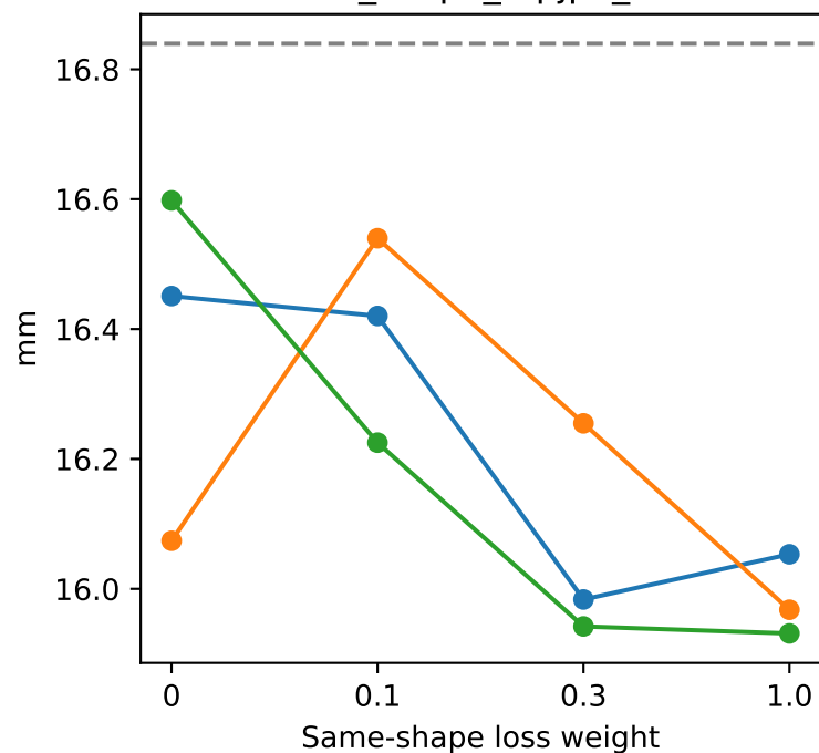
same_shape_mpjpe_mm
