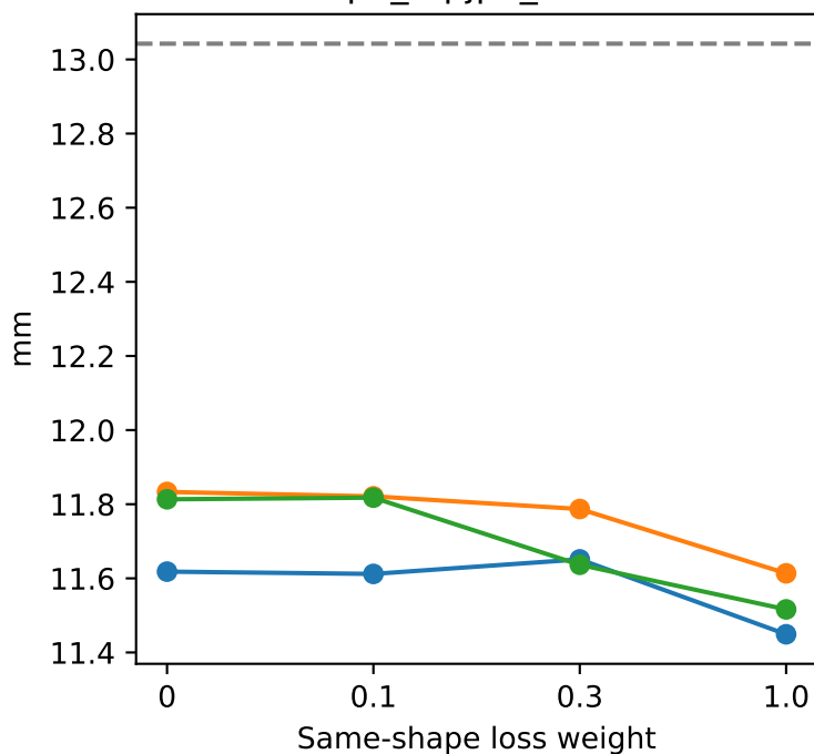
pa_mpjpe_mm
