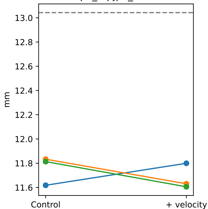
pa_mpjpe_mm
