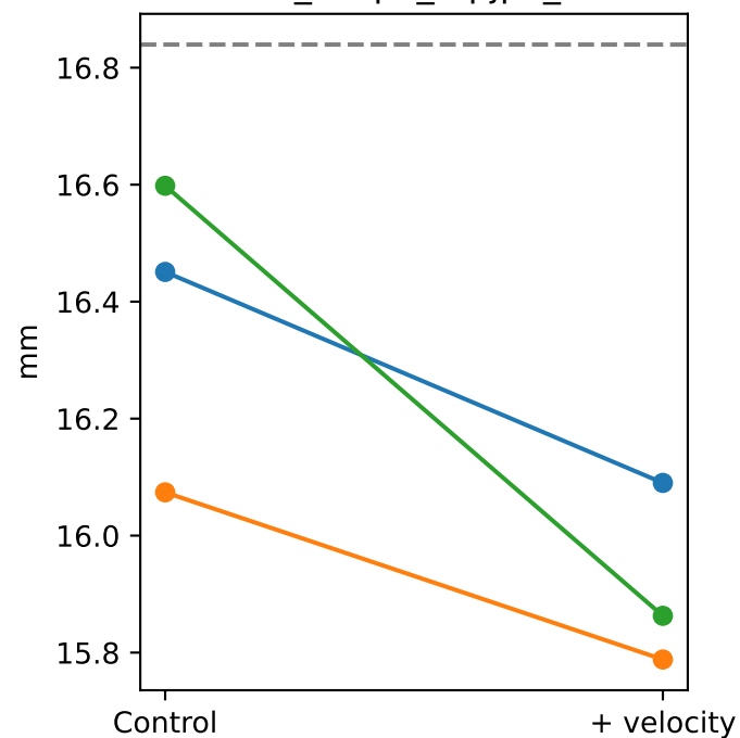
same_shape_mpjpe_mm
