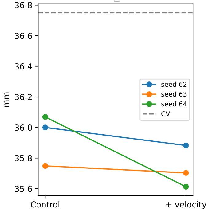
fk22_mm
